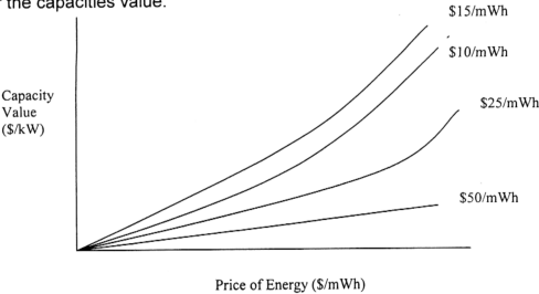
Figure 9.4: Capacity Value versus Fuel Price
