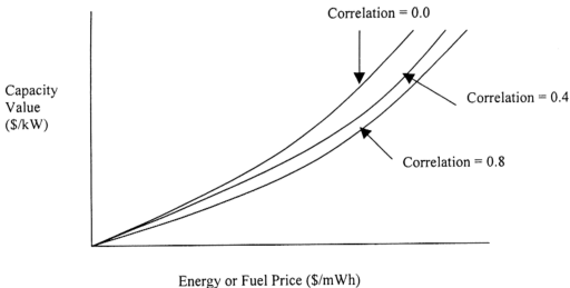
Figure 9.6 : Capacity Value versus Correlation of Energy and Fuel Prices
