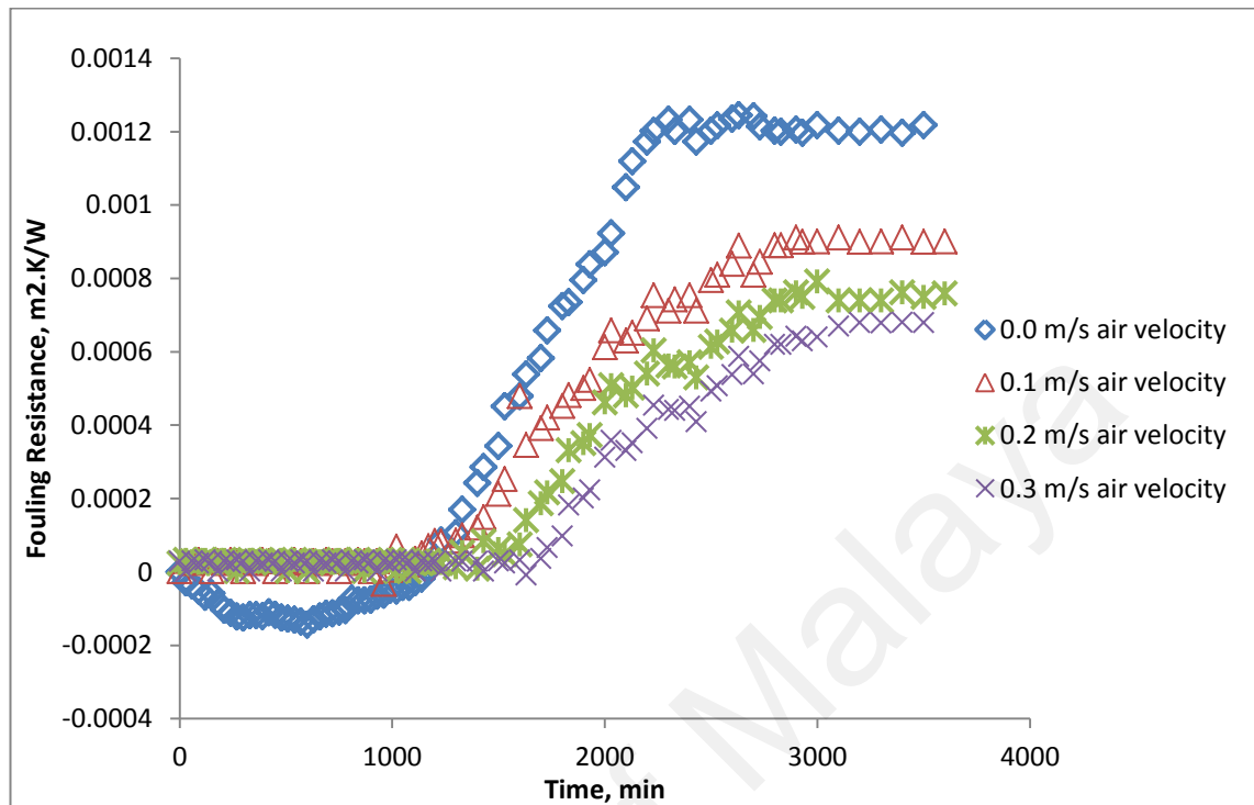
Figure 7.26: Fouling resistance as the function of time based on different air velocity input at constant \Delta T = 15^\circ\text{C} , 0.2 m/s water flow and 500 mg/l concentration.
