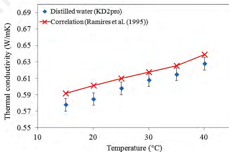
Figure 3.8: Comparison between distilled water and previous data.
