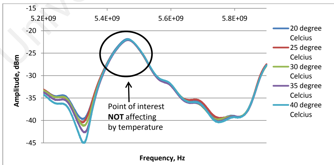
Figure 7.19: S_{21} spectrum signal under effect of temperature from 5.2-5.9 GHz.
