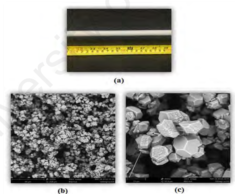
Figure 4.17: Image (a) and crystal morphology (b & c) of calcium carbonate formation at 500 mg/l, 50 °C and 25 °C at hot and solution inlet respectively and 0.15 m/s solution flow velocity.
