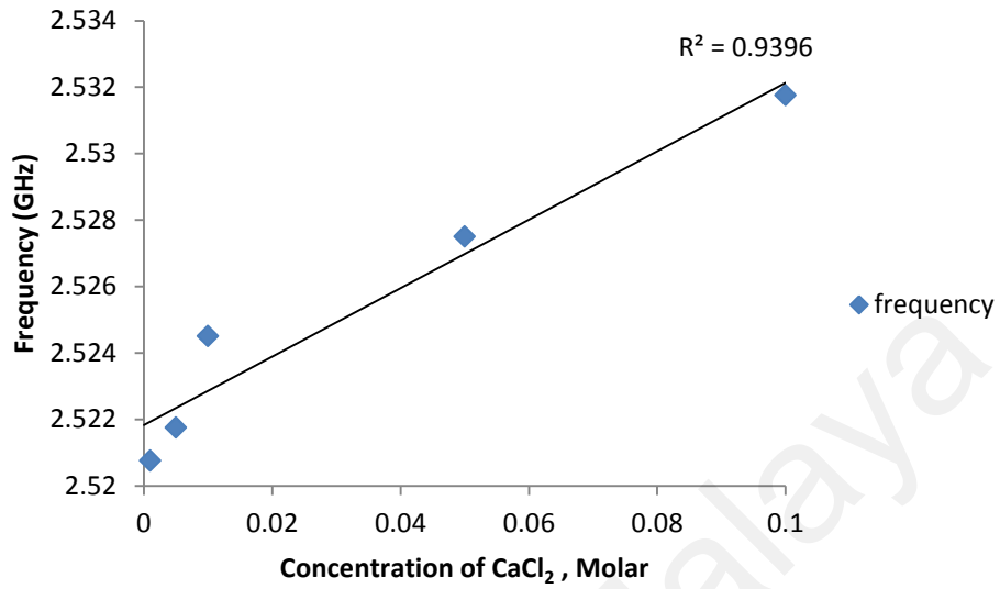
Figure 6.5: Frequency shifts at varying \text{CaCl}_2 concentrations.
