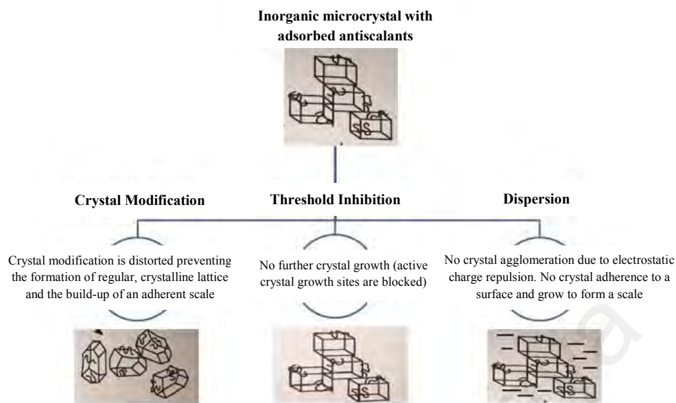
Figure 2.11: Summary of primary chemical scale inhibition mechanism (Nguyen, Roddick, & Fan, 2012).
