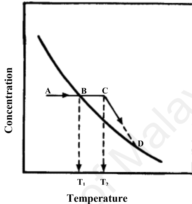
Figure 2.5: Effect of temperature on an inverse solubility salt solution (Bott, 1995).
