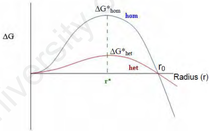
Figure 2.7: Free energy changes associated with homogeneous and heterogeneous mechanism (Brar, France, & Smirniotis, 2001).
