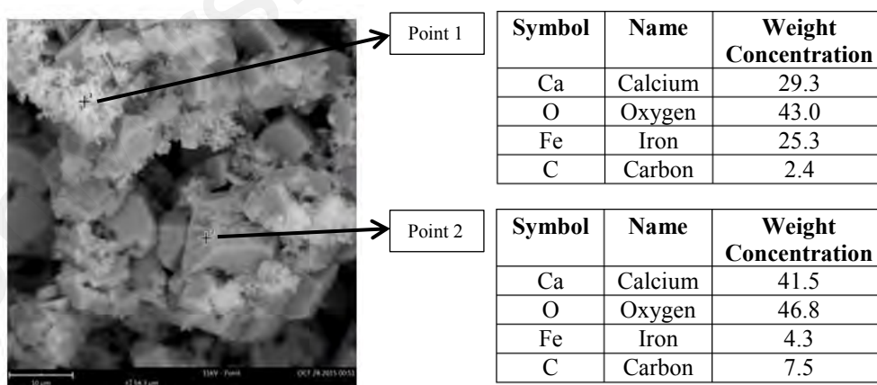
Figure 4.22: SEM and EDS analyses of the deposited materials on carbon steel.
