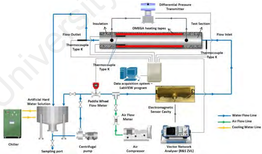
Figure 7.2: Schematic layout of two-phase flow experimental system.
