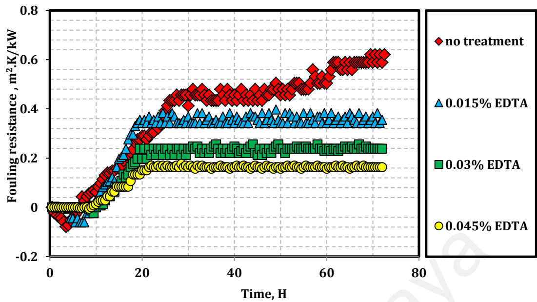
Figure 5.10: Fouling resistances under influence of EDTA additive at inlet temperature of 60 °C with 300 mg/l CaCO 3 .
