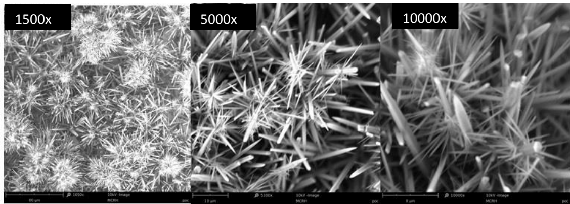
Figure 4.25: SEM images of 1500x – 10000x of calcium carbonate crystal under PWT case.
