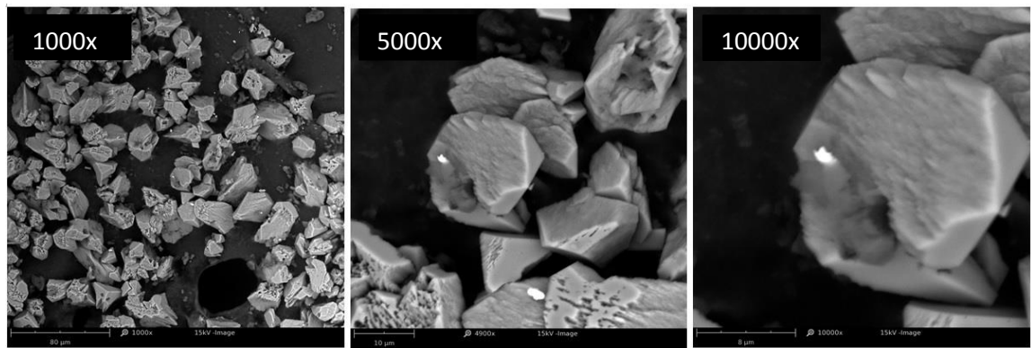
Figure 5.16: Crystal morphology of \text{CaCO}_3 under effect of 0.03wt% additives concentration.
