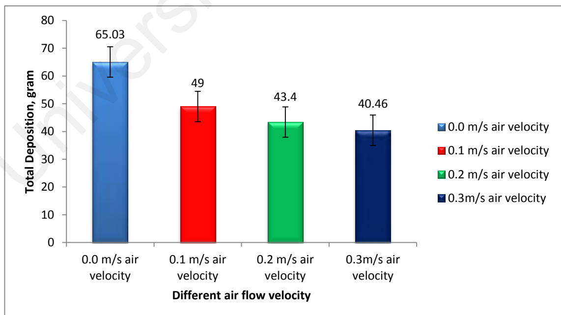
Figure 7.27: Total deposition on test section surface under effect of air velocity input, at constant \Delta T = 15^\circ\text{C} , 0.2 m/s water flow and 500 mg/l concentration.
