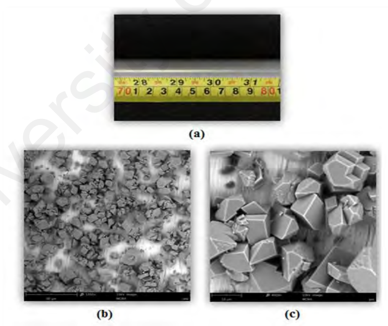
Figure 4.15: Image (a) and crystal morphology (b & c) of calcium carbonate formation at 300 mg/l, 50 °C and 25 °C at hot and solution inlet respectively and 0.15 m/s solution flow velocity.
