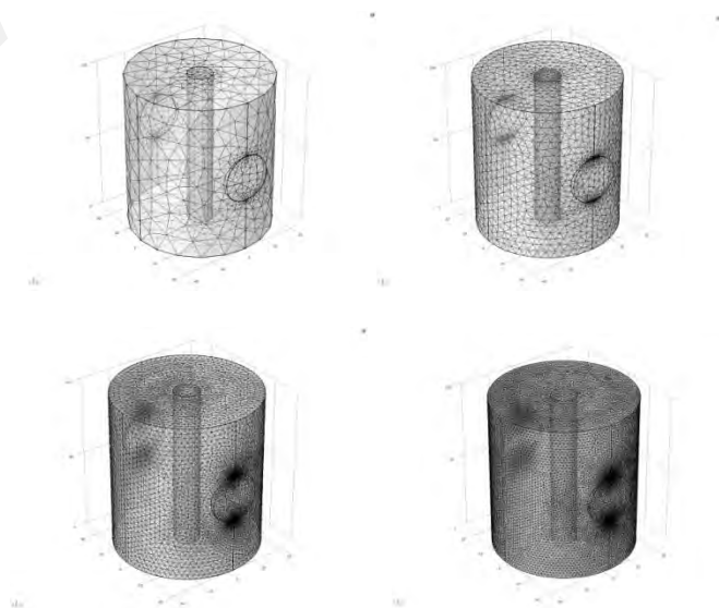
Figure 6.14: Different meshes used in this simulation, (a) coarse mesh, (b) normal mesh, (c) fine mesh, and (d) extra fine mesh
