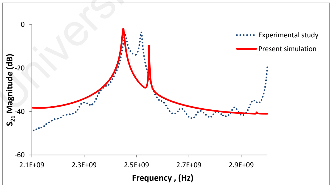
Figure 6.16: Comparison of simulated frequency spectrum data with experimental frequency spectrum data.
