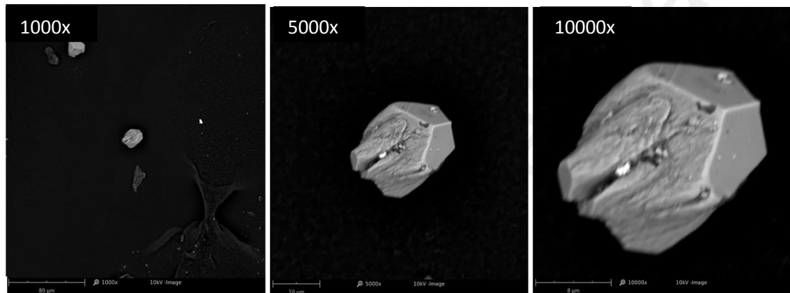
Figure 5.17: Crystal morphology of \text{CaCO}_3 under effect of 0.045wt% additives concentration.
