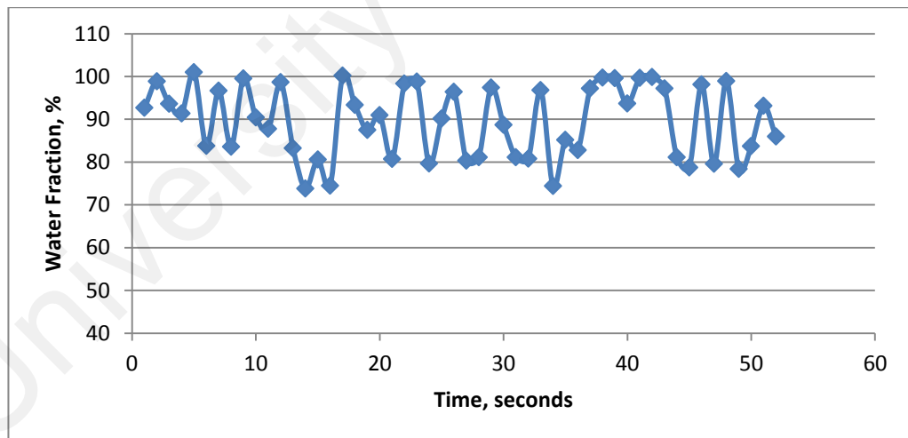
Figure 7.22: S_{21} signal under effect of 0.2 m/s water velocity and 0.1 m/s air velocity (Plug Flow)
