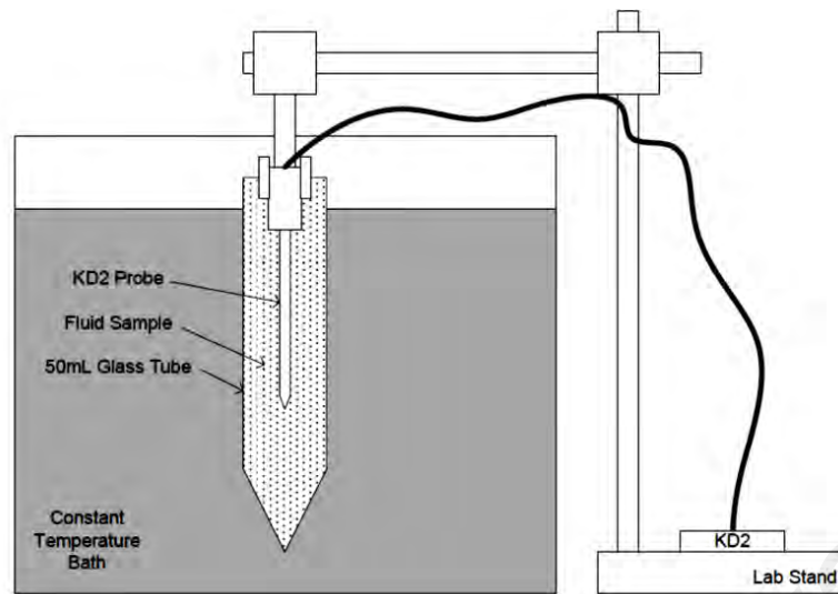
Figure 3.7: Schematic Setup of KD2 Thermal Properties Analyser.
