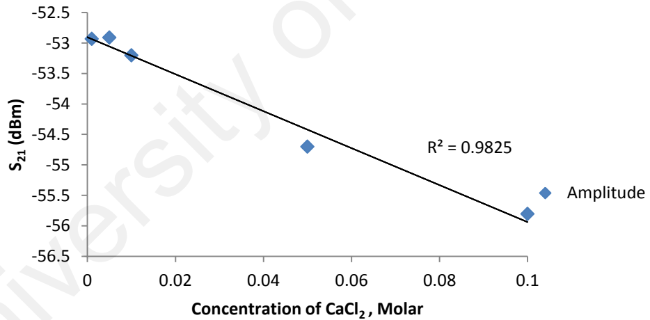
Figure 6.6: Amplitude changes for varying \text{CaCl}_2 concentration.
