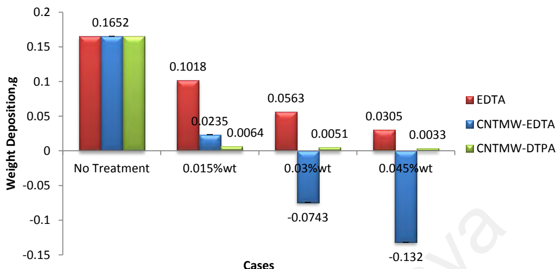
Figure 5.9: Deposition of fouling under effect of concentration at inlet temperature of 60 °C for MWCNT-DTPA.
