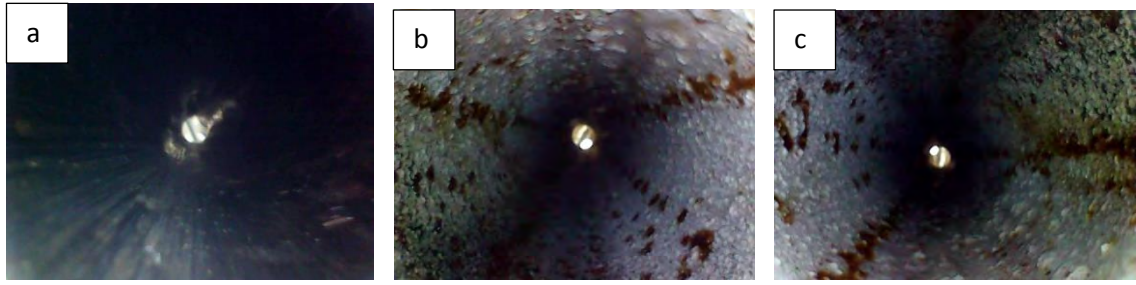
Figure 7.28: Deposition on test section surface under effect of air velocity input [(a) clean pipe surface, (b) 0.0 m/s air velocity & (c) 0.3 m/s air velocity], at constant \Delta T = 15^\circ\text{C} , 0.2 m/s water flow and 500 mg/l concentration .
