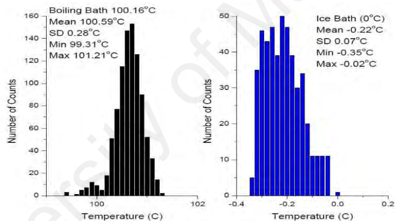
Figure 3.22: Thermocouple testing.
