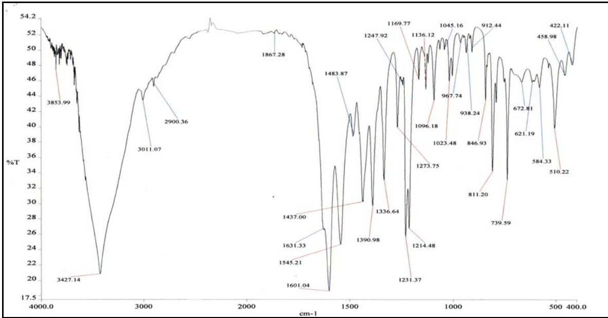
Figure 4.6 IR spectrum of Ni_4F_2 -HapIH
