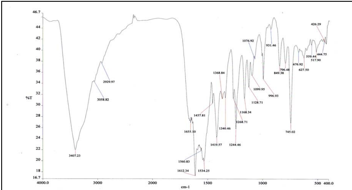
Figure 4.8 IR spectrum of 5- \text{CH}_3 -2-HapIH
