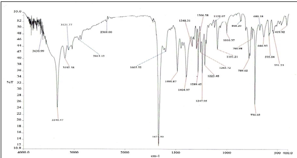
Figure 4.8 IR spectrum of 5- \text{CH}_3 -2-HapIH
