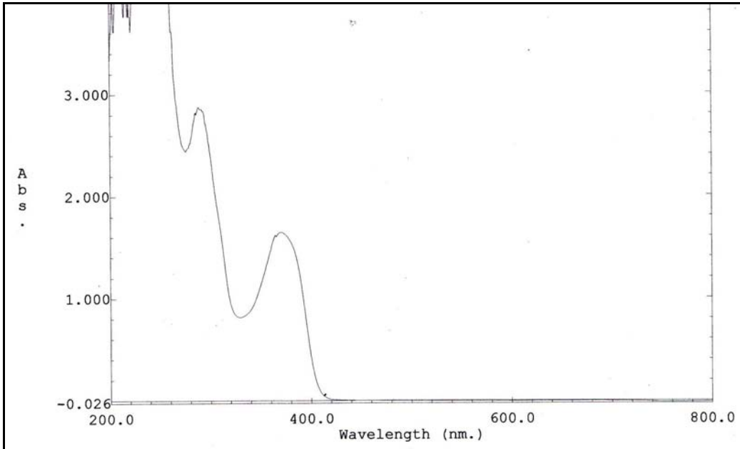
Figure 4.19 UV visible spectrum of Ni 2 -HapIH
