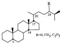
VIII. \alpha\beta -Steranes
