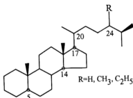
VII. \alpha\alpha -Steranes
