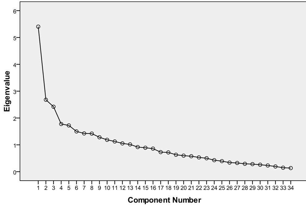
Scree Plot
