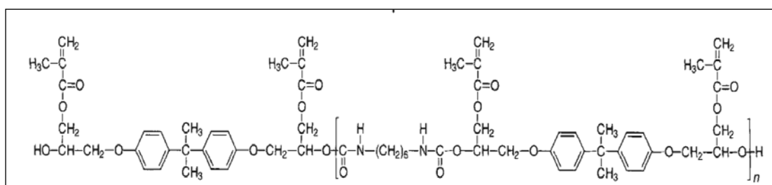
Figure 2.6 Schematic representation of the UDMA oligomer used in Ful-Fil composite (Peutzfeldt, 1997)
