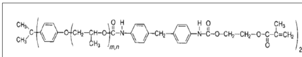
Figure 2.5 Schematic representation of the UDMA used in Fotofil composite (Peutzfeldt, 1997)
