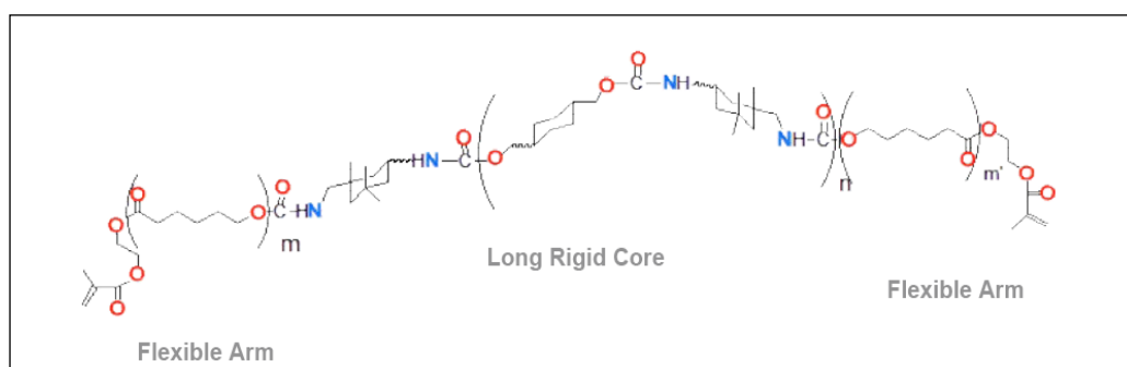
Figure 2.7 Schematic representation of the UDMA used in Kalore composite
