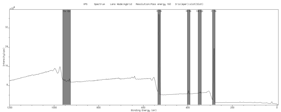
Figure C3 XPS wide spectra of PSMC after Cu(II) biosorption
