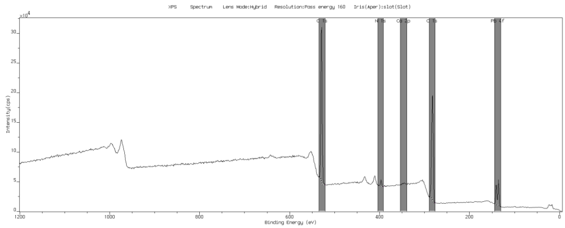
Figure C2 XPS wide spectra of PSMC after Pb(II) biosorption
