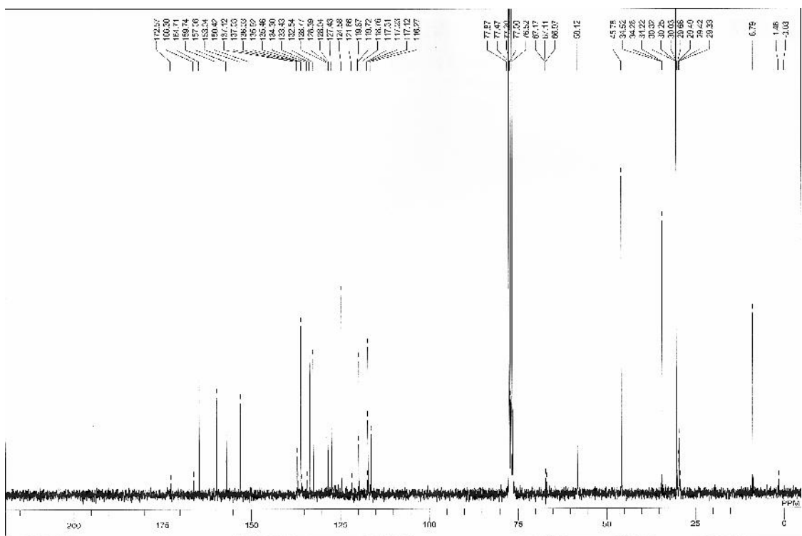
^{13}\text{C} NMR spectrum of \{N'-(2\text{-oxidobenzylidene})[2-(3,5\text{- di-}i\text{-tert-butyl-4-hydroxybenzyl)-\text{sulfanyl}]acetato\text{hydrazidato}\} dimethyltin(IV), DA1
