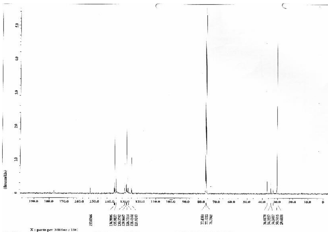
^{13}\text{C} NMR spectrum of catena -poly{ bis [triphenyltin(IV)[2-(3,5-di- tert -butyl-4-hydroxybenzyl)sulfanyl]acetate]}, AC1
