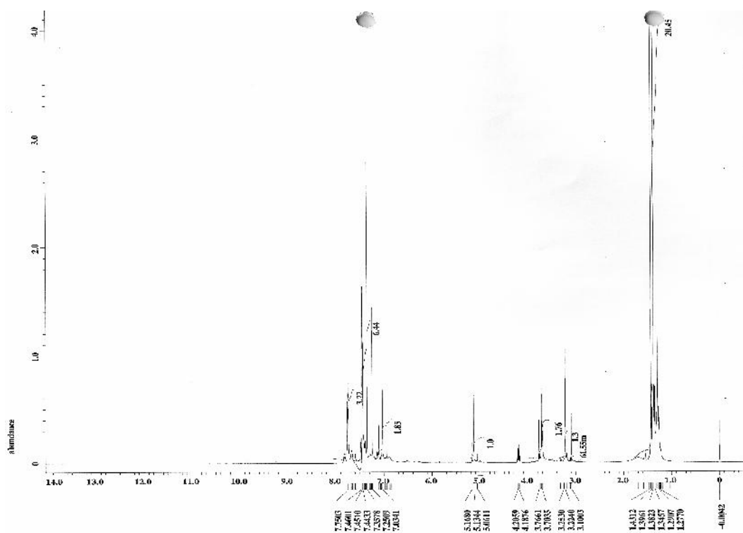
^1\text{H} NMR spectrum of catena -poly{ bis [triphenyltin(IV)[2-(3,5-di- tert -butyl-4-hydroxybenzyl)sulfanyl]acetate]}, AC1
