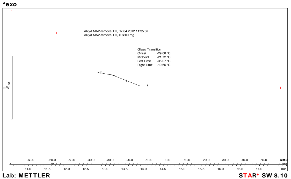
DSC thermogram of Alkyd MA2
