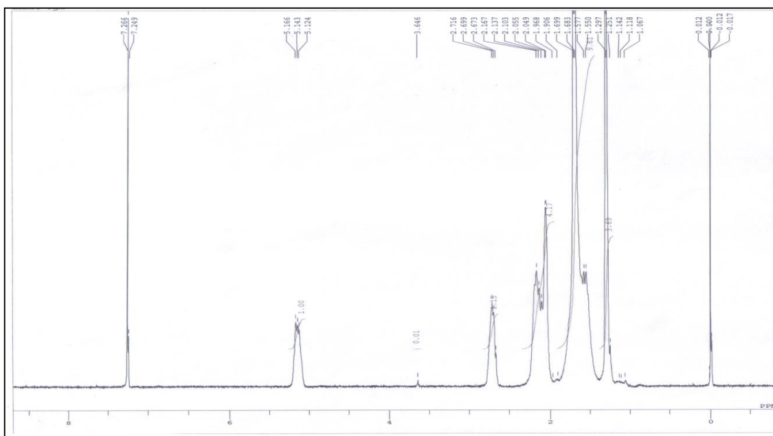
^1\text{H-NMR} spectrum of ENR50
