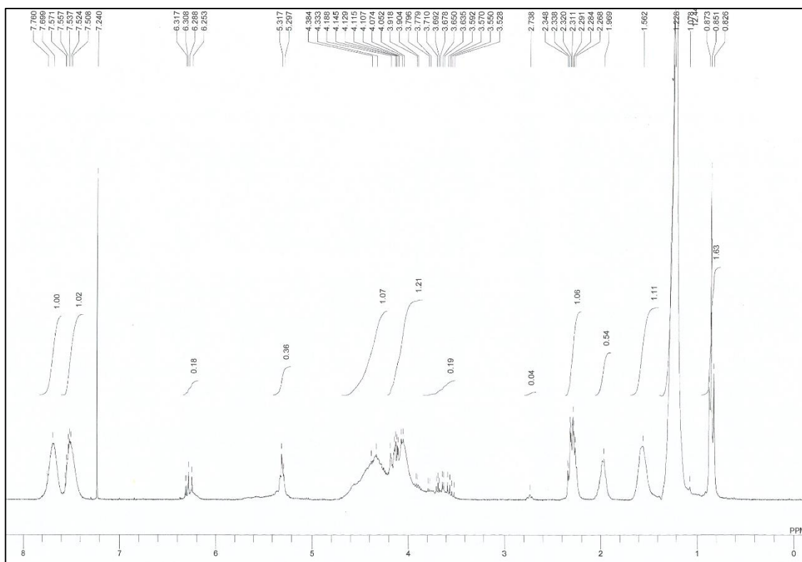
1 H-NMR spectrum of AlkydMA1
