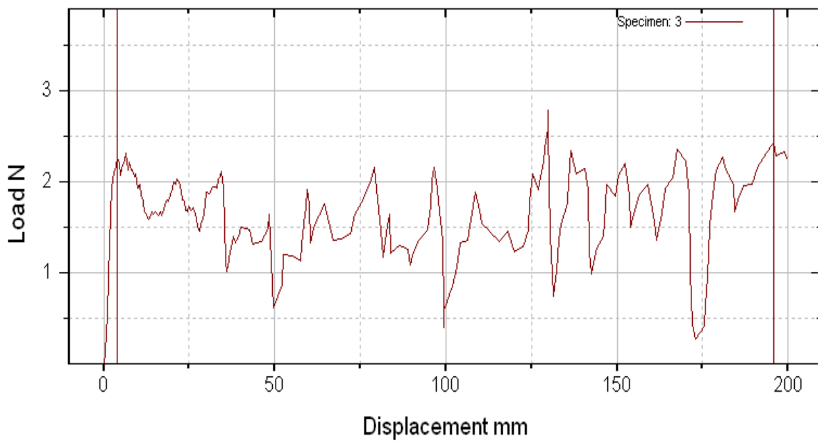
Figure 2(a): A Peel test curve of commercial PSA tapes Loytape
