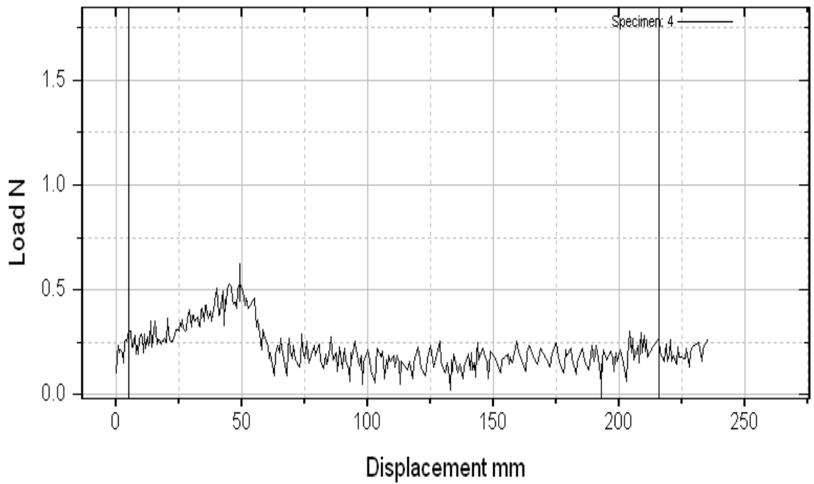
Figure 1(b): A Peel test curve of sample Alk-45 PSA tapes
