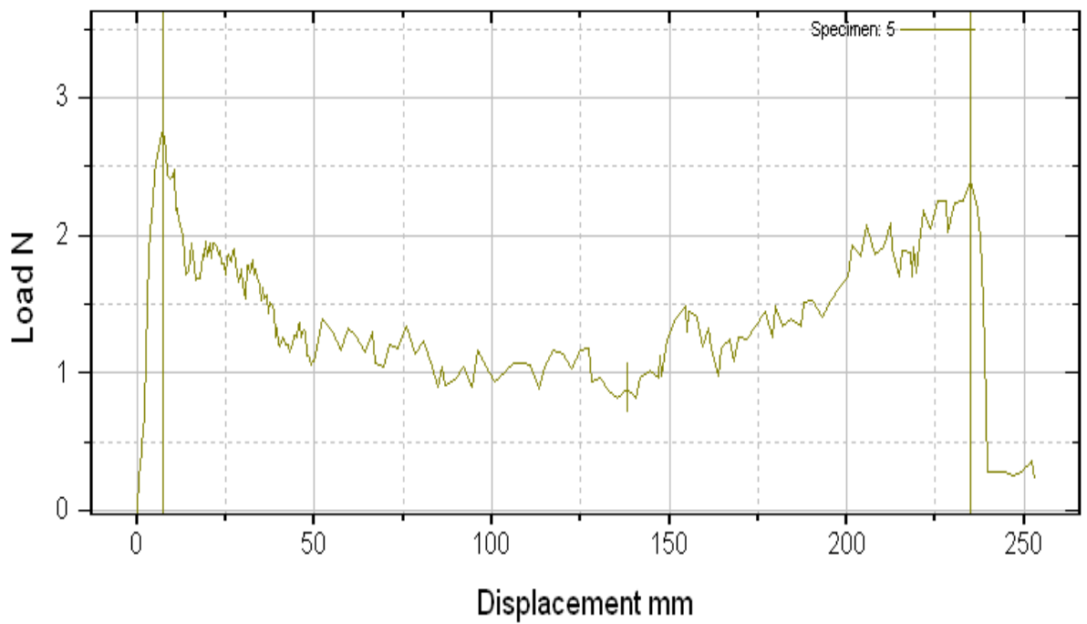
Figure 1(d): A Peel test curve of sample Alk-47 PSA tapes
