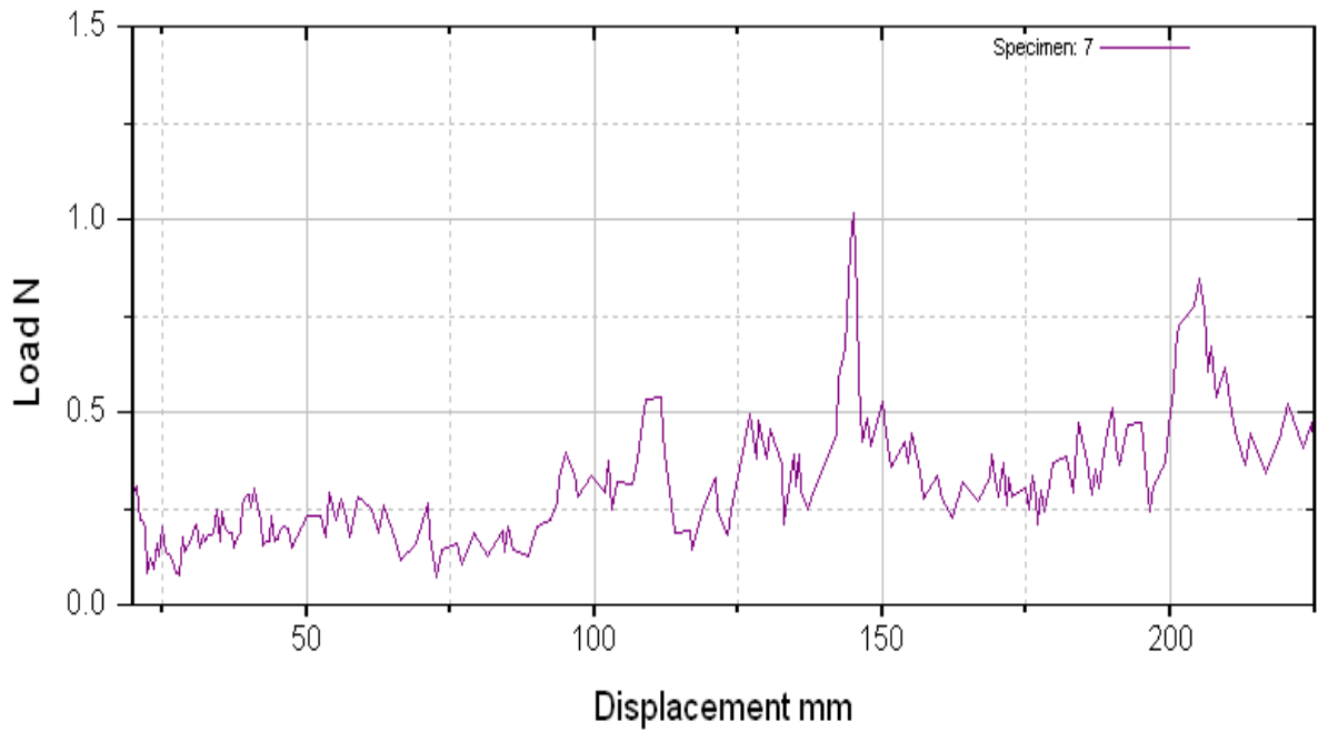
Figure 1(a): A Peel test curve for pure Alk-47
