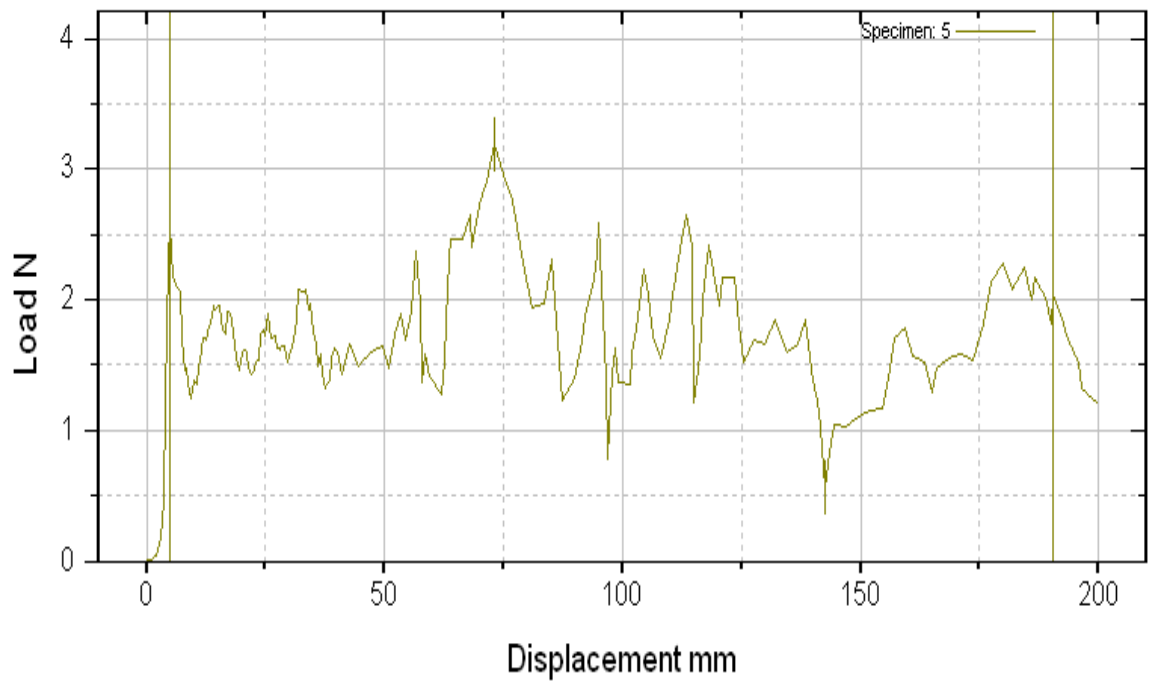
Figure 1(c): A Peel test curve of commercial PSA tapes Toyo
