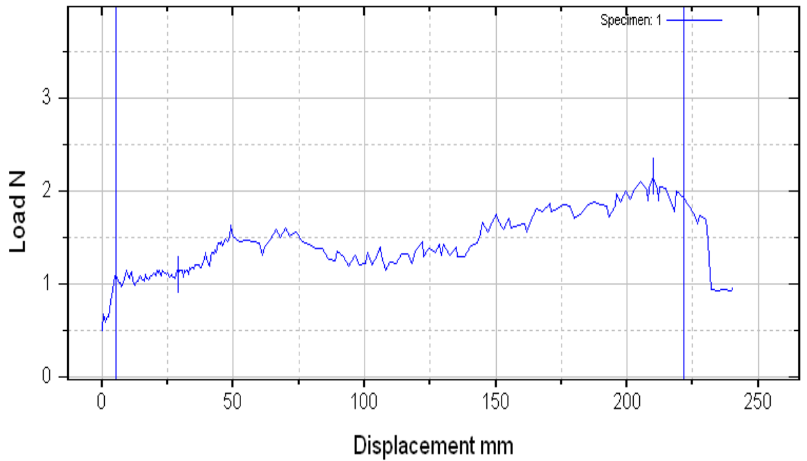
Figure 1(a): A Peel test curve of sample Alk-47 PSA tapes
