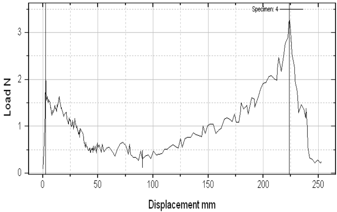
Figure 1(c): A Peel test curve of sample Alk-47 PSA tapes
