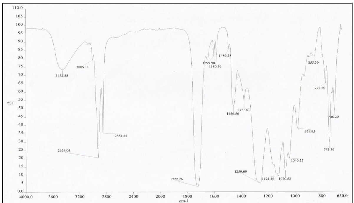
Figure 2: FTIR spectra of Alk-47
