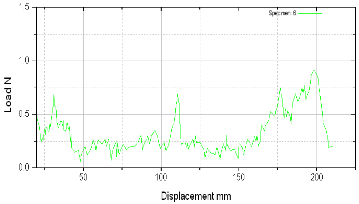
Figure 1(c): A Peel test curve for pure Alk-47
