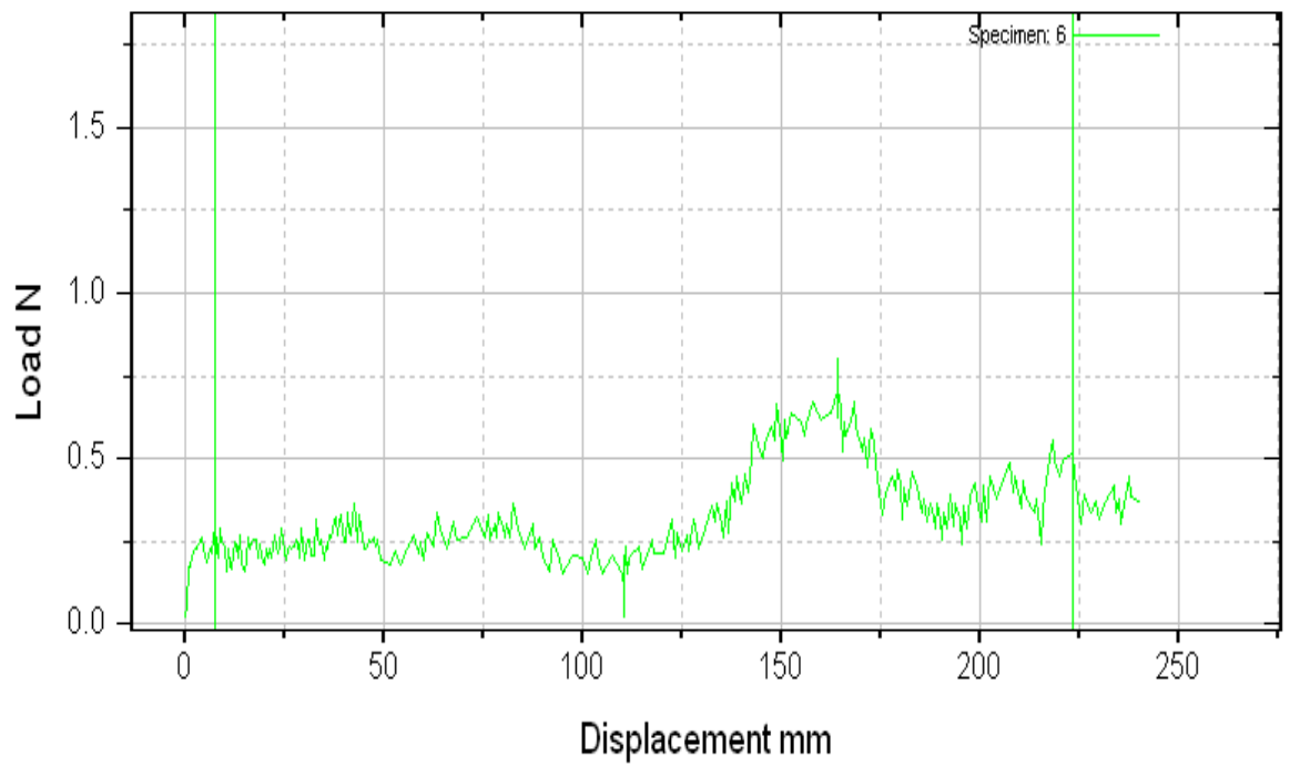
Figure 1(d): A Peel test curve of sample Alk-45 PSA tapes
