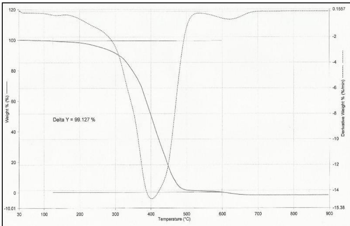
Figure 3: TGA thermogram of Alk-65
