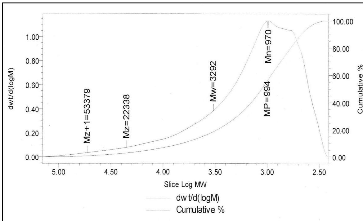
Figure 3: GPC chromatogram of Alk-65
