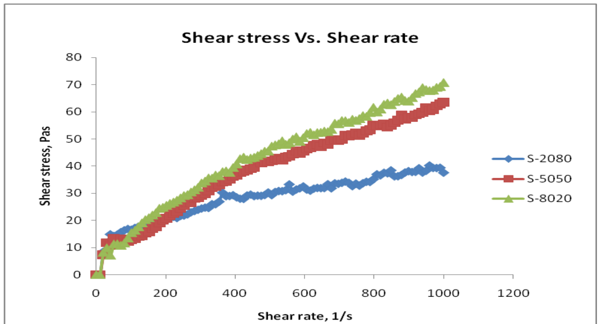
Figure 2: Shear stress Vs. Shear rate for Alk-45 emulsion at different surfactant ratio
