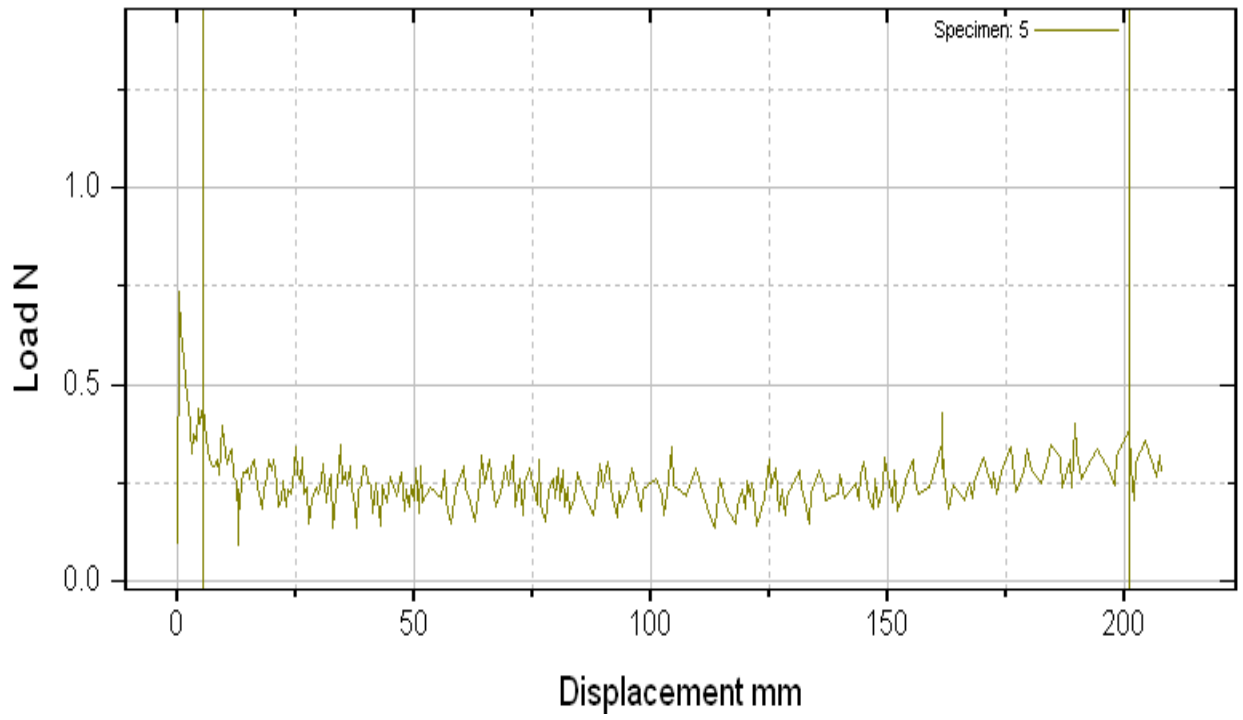
Figure 1(c): A Peel test curve for pure Alk-65
