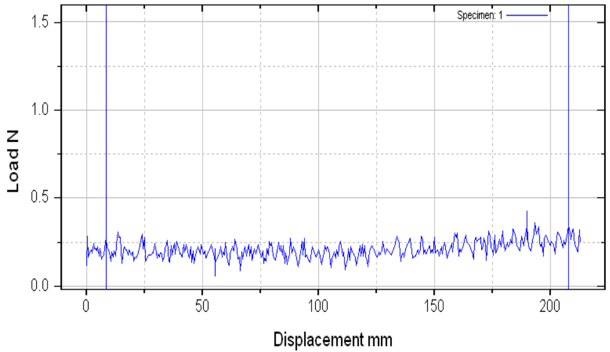
Figure 1(a): A Peel test curve for pure Alk-65
