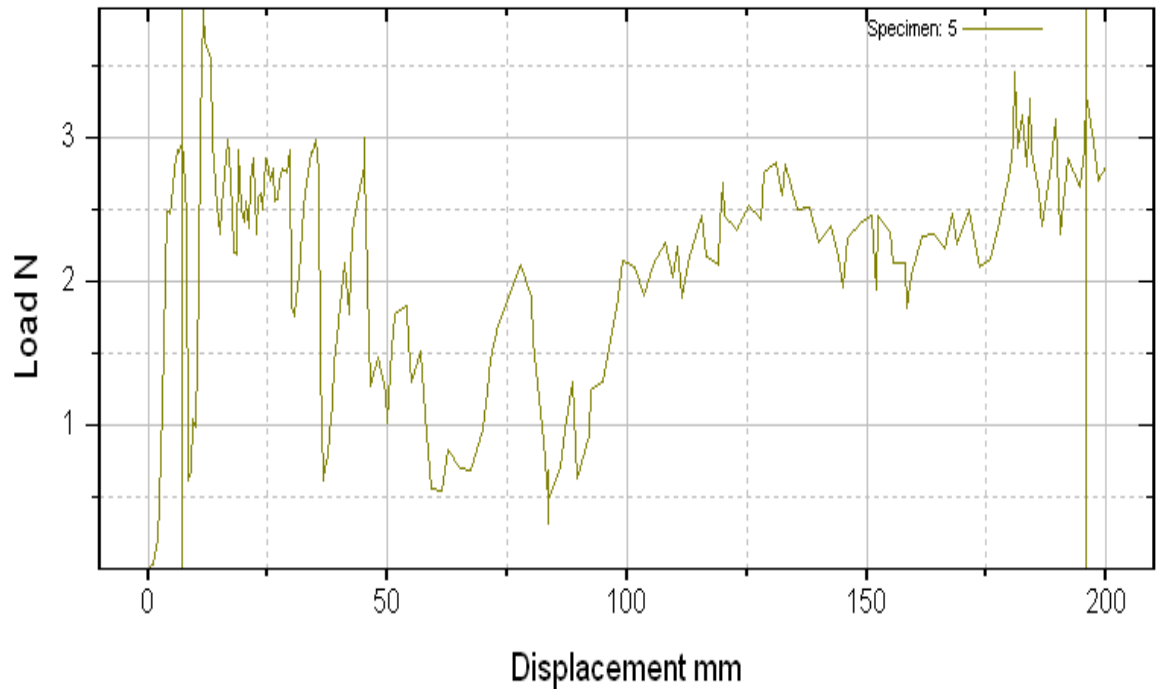
Figure 2(b): A Peel test curve of commercial PSA tapes Loytape
