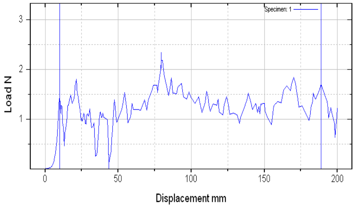
Figure 3(a): A Peel test curve of commercial PSA tapes ESI
