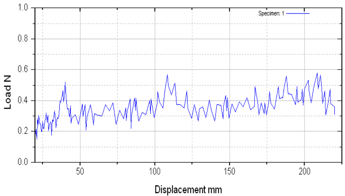
Figure 1(b): A Peel test curve for pure Alk-47
