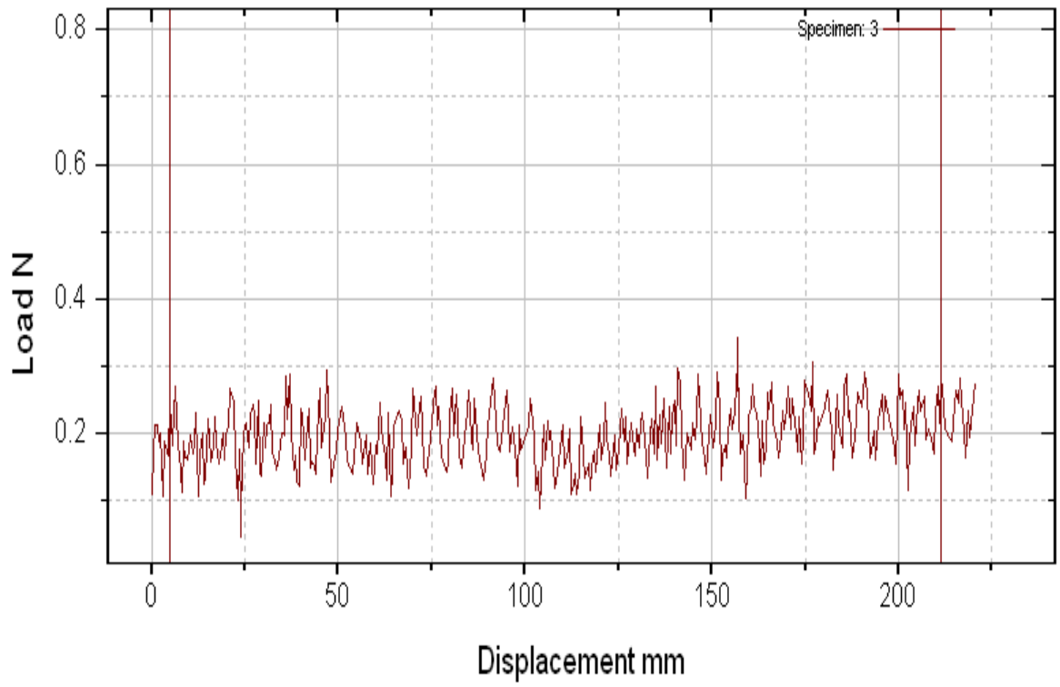
Figure 1(e): A Peel test curve of sample Alk-65 PSA tapes
