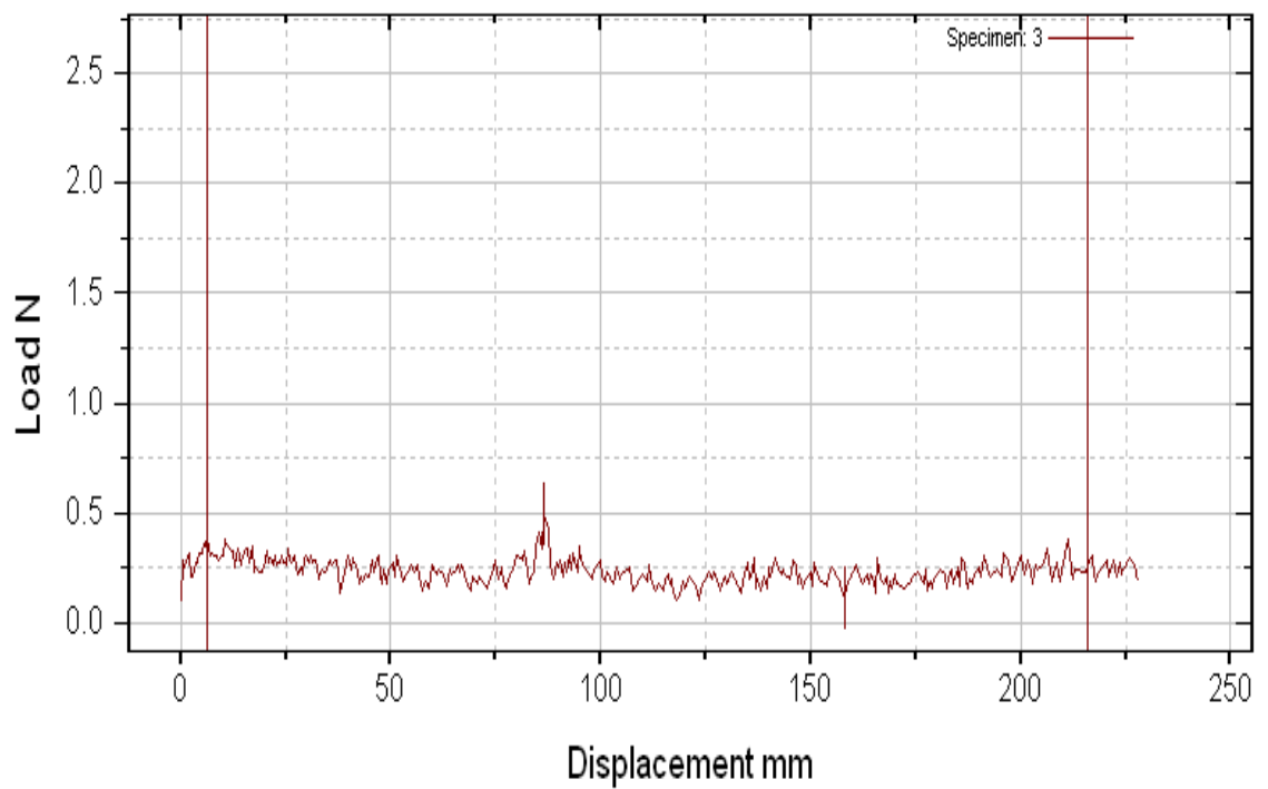
Figure 1(b): A Peel test curve of sample Alk-65 PSA tapes
