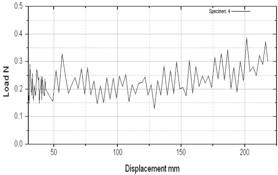
Figure 1(c): A Peel test curve for pure Alk-45
