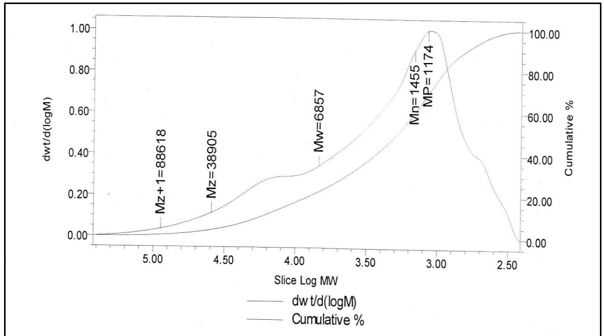
Figure 1: GPC chromatogram of Alk-45
