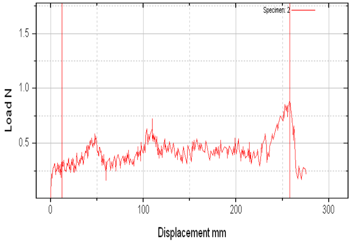
Figure 1(e): A Peel test curve of sample Alk-45 PSA tapes
