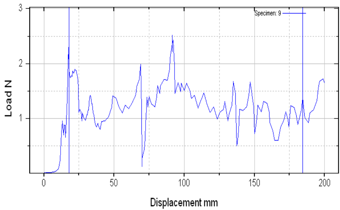
Figure 3(c): A Peel test curve of commercial PSA tapes ESI
