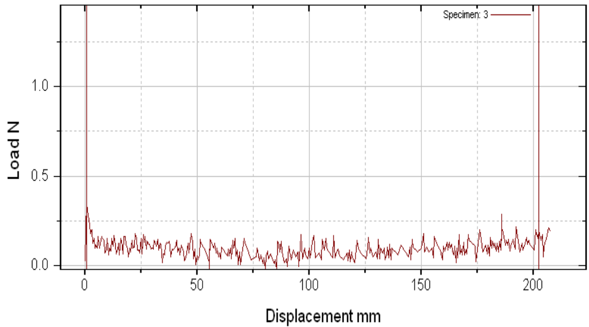
Figure 1(b): A Peel test curve for pure Alk-65
