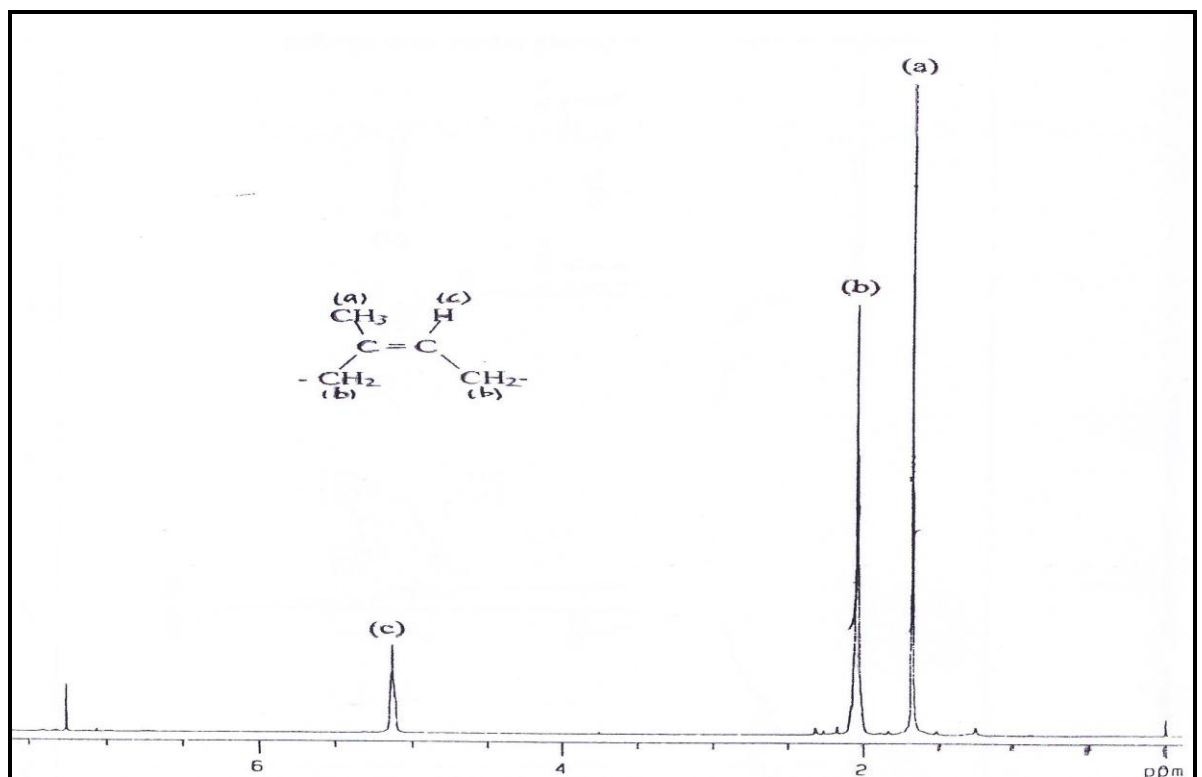
Figure 2: NMR spectrum of natural rubber
