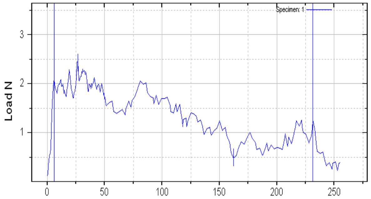
Figure 1(e): A Peel test curve of sample Alk-47 PSA tapes
