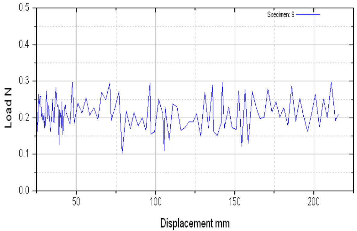
Figure 1(a): A Peel test curve for pure Alk-45
