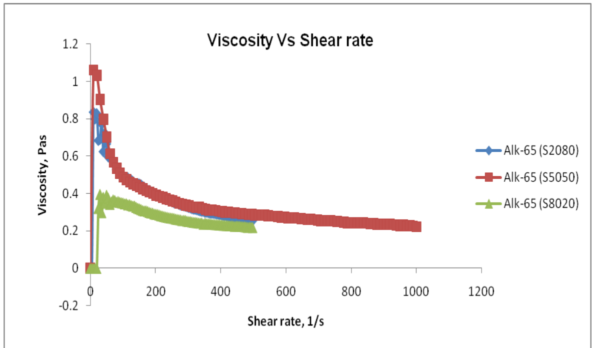
Figure 5: Viscosity Vs Shear rate of Alk-65 emulsion at different surfactant ratio
