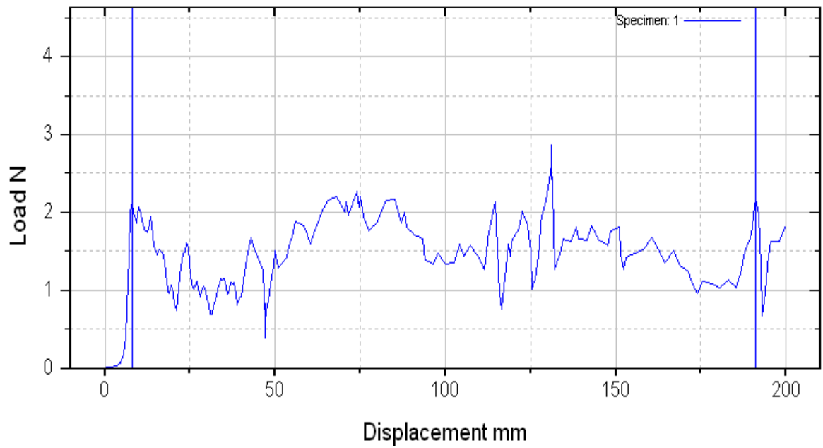
Figure 1(a): A Peel test curve of commercial PSA tapes Toyo
