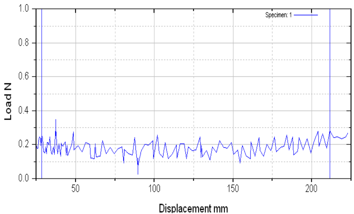
Figure 1(b): A Peel test curve for pure Alk-45
