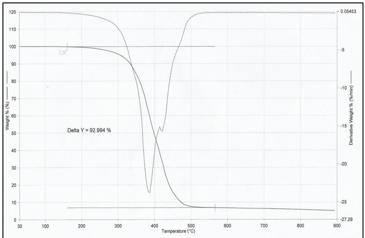
Figure 2: TGA thermogram of Alk-47
