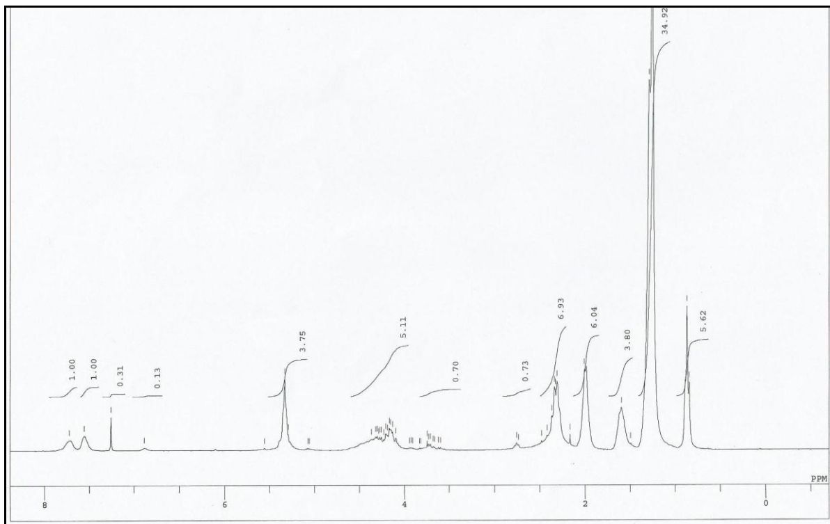
Figure 3: NMR spectra of Alk-65
