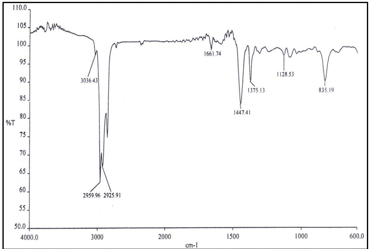
Figure 1: FTIR spectrum of Natural rubber
