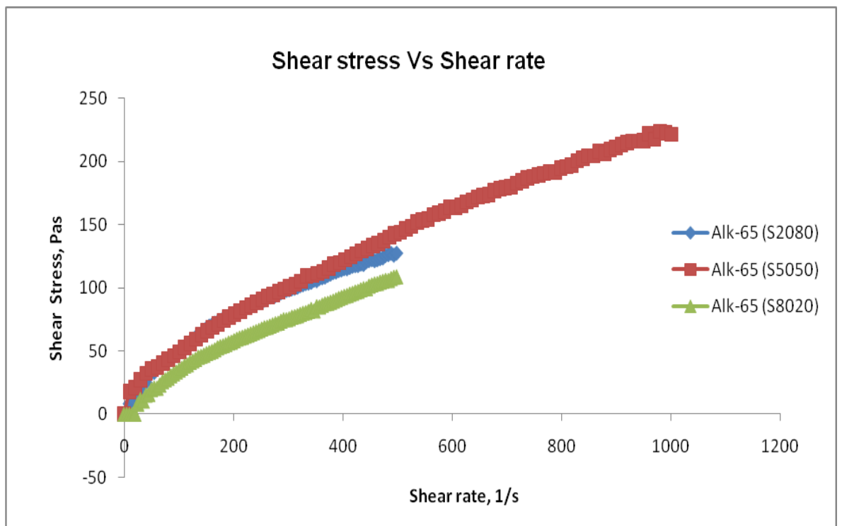
Figure 6: Shear stress Vs Shear rate of Alk-65 emulsion at different surfactant ratio
