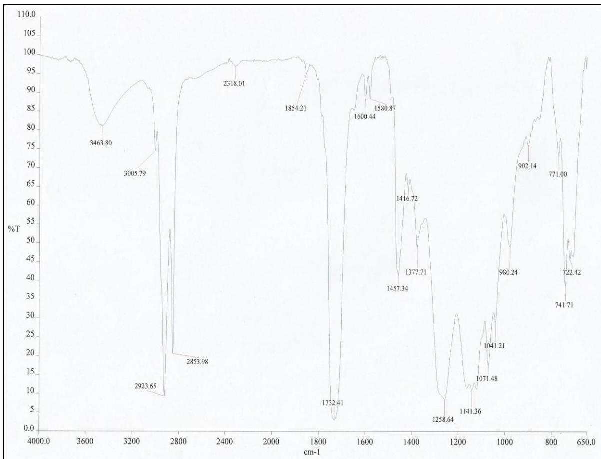
Figure 3: FTIR spectra of Alk-65
