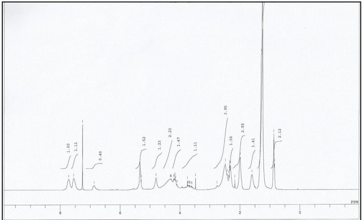
Figure 2: NMR spectra of Alk-47
