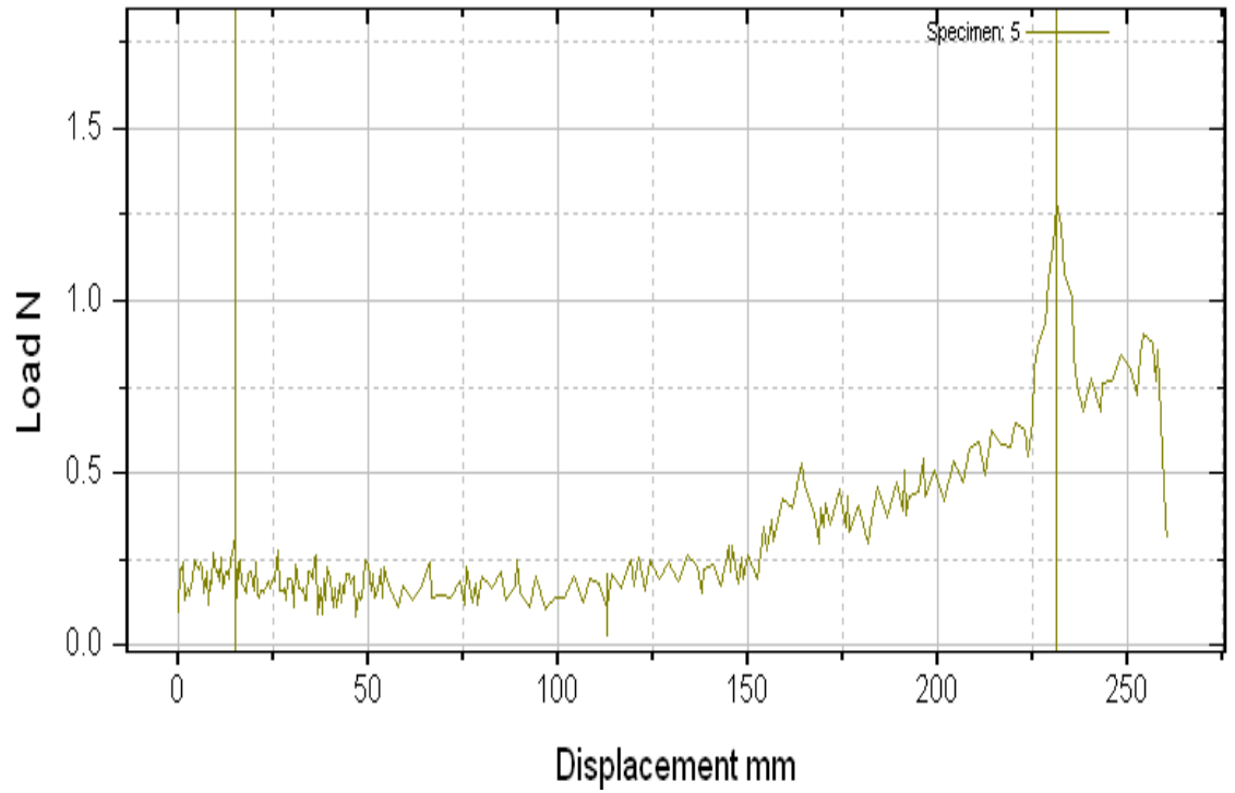
Figure 1(a): A Peel test curve of sample Alk-45 PSA tapes
