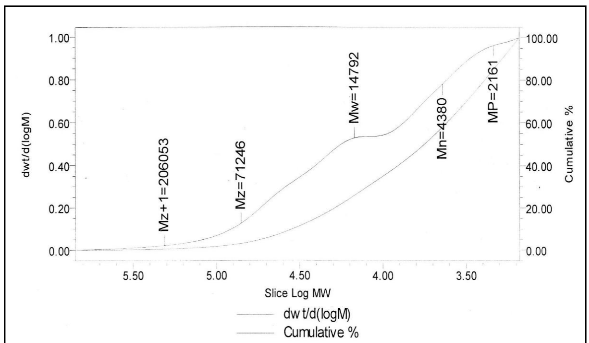
Figure 2: GPC chromatogram of Alk-47
