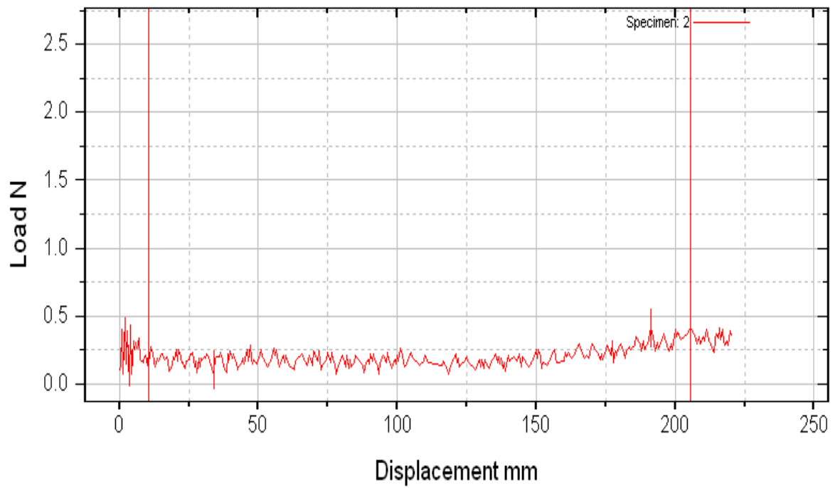
Figure 1(a): A Peel test curve of sample Alk-65 PSA tapes
