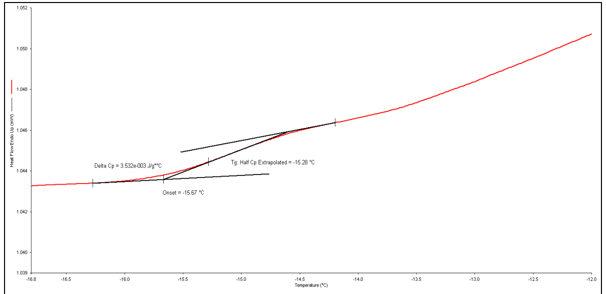
Figure 1: DSC trace of Alk-45
