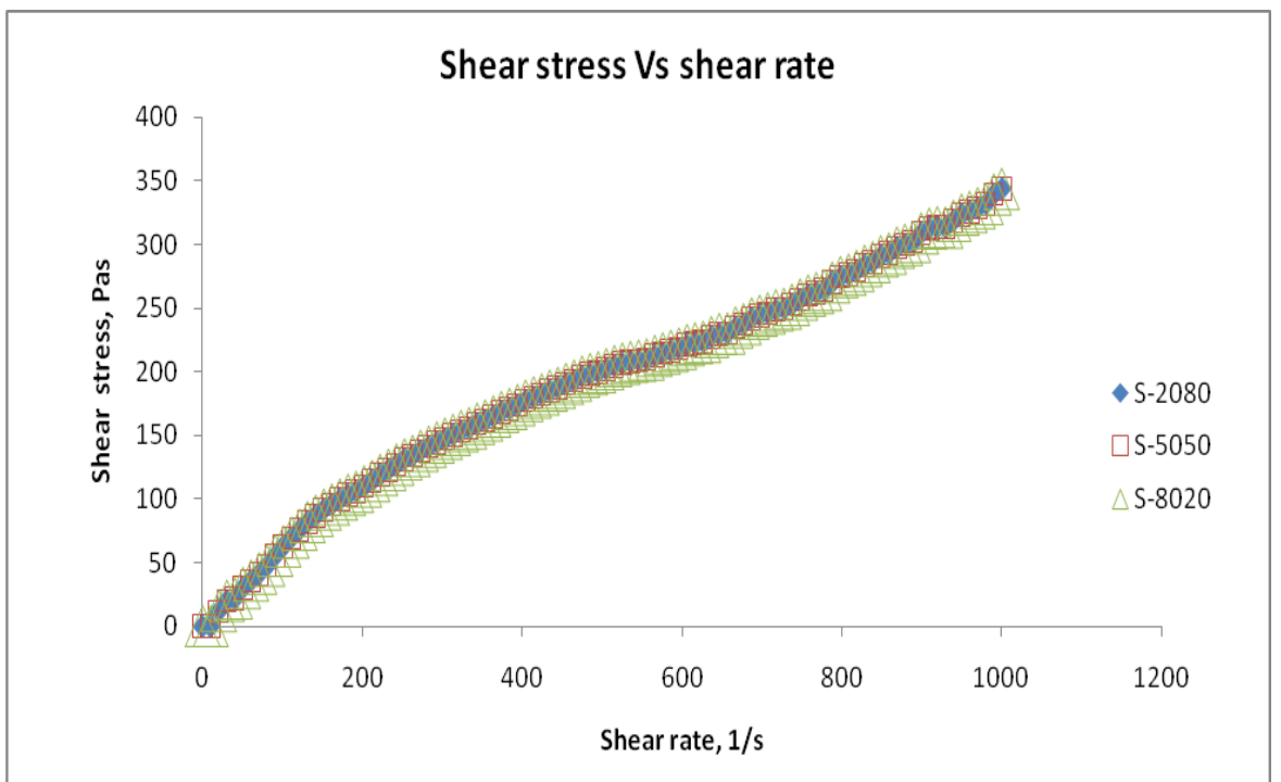
Figure 4: Shear stress Vs. Shear rate for alk-47 emulsion at different surfactant ratio
