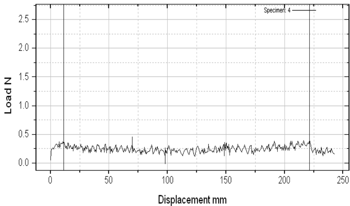
Figure 1(c): A Peel test curve of sample Alk-65 PSA tapes
