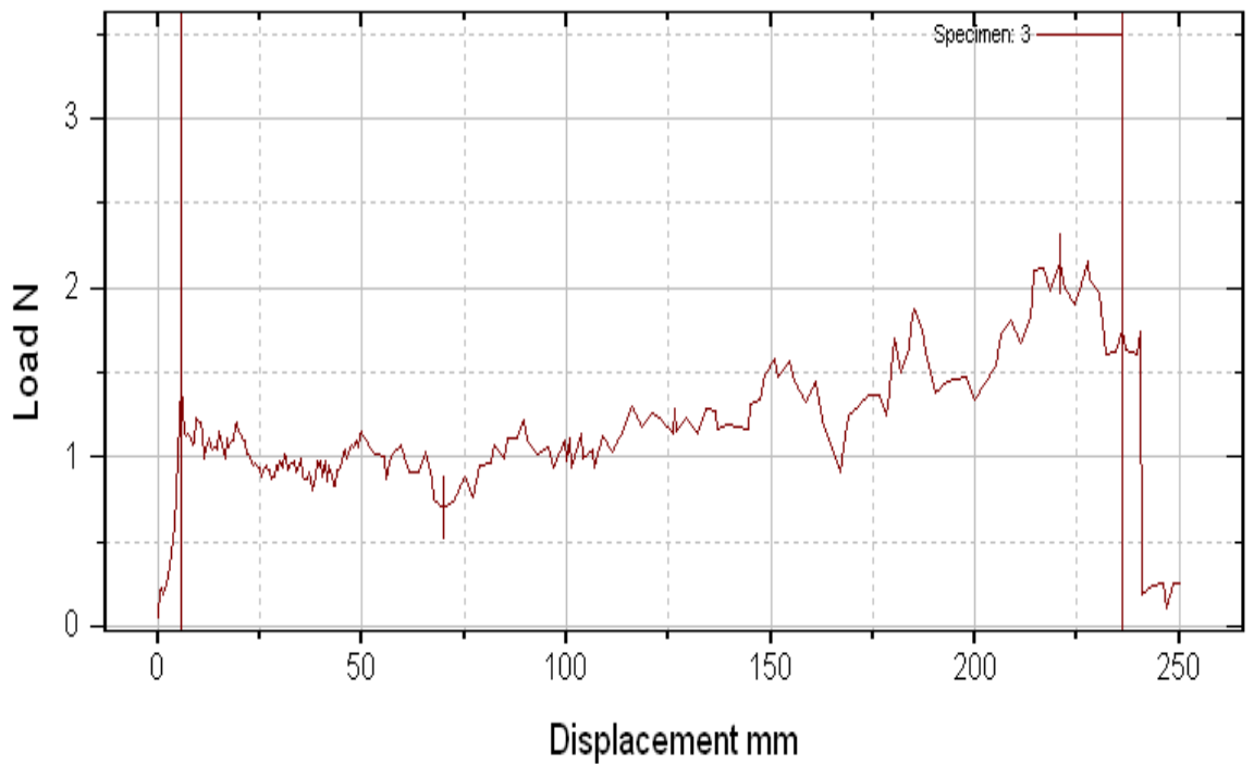
Figure 1(b): A Peel test curve of sample Alk-47 PSA tapes
