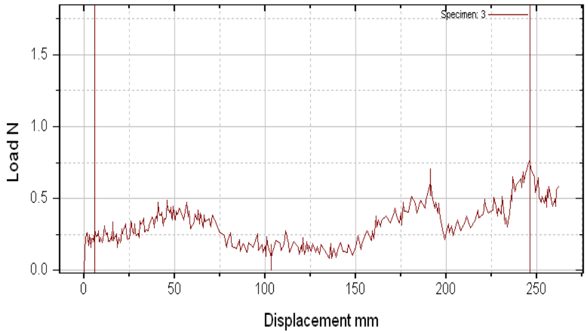
Figure 1(c): A Peel test curve of sample Alk-45 PSA tapes
