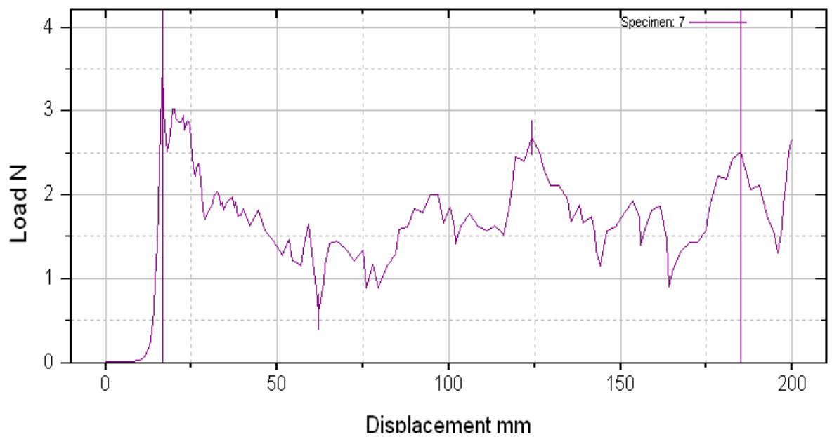
Figure 1(b): A Peel test curve of commercial PSA tapes Toyo
