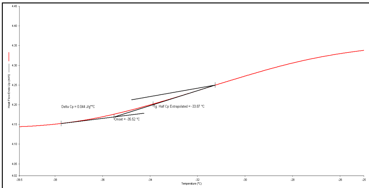
Figure 3: DSC trace of Alk-65
