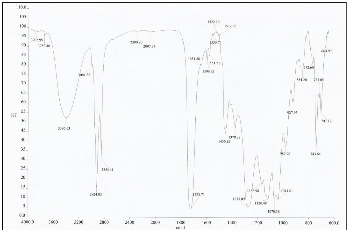
Figure 1: FTIR spectra of Alk-45
