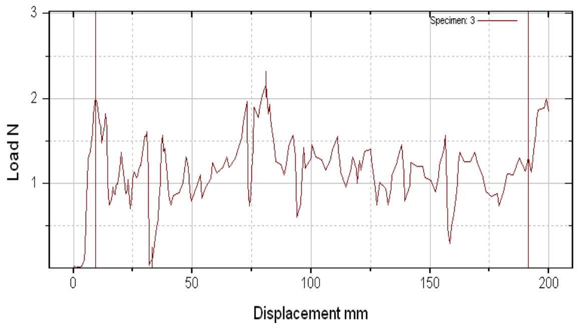
Figure 3(b): A Peel test curve of commercial PSA tapes ESI
