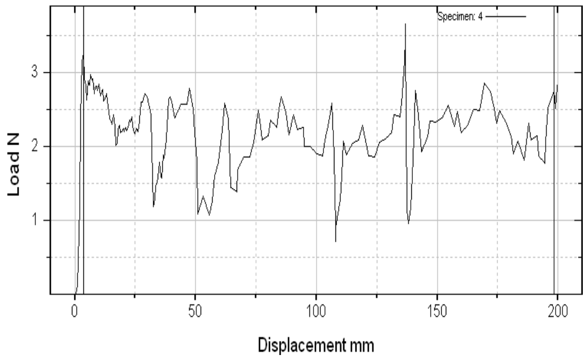
Figure 2(c): A Peel test curve of commercial PSA tapes Loytape
