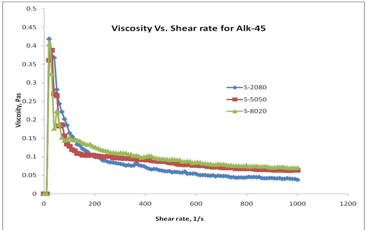
Figure 1: Viscosity Vs Shear rate for Alk-45 emulsion at different surfactant ratio
