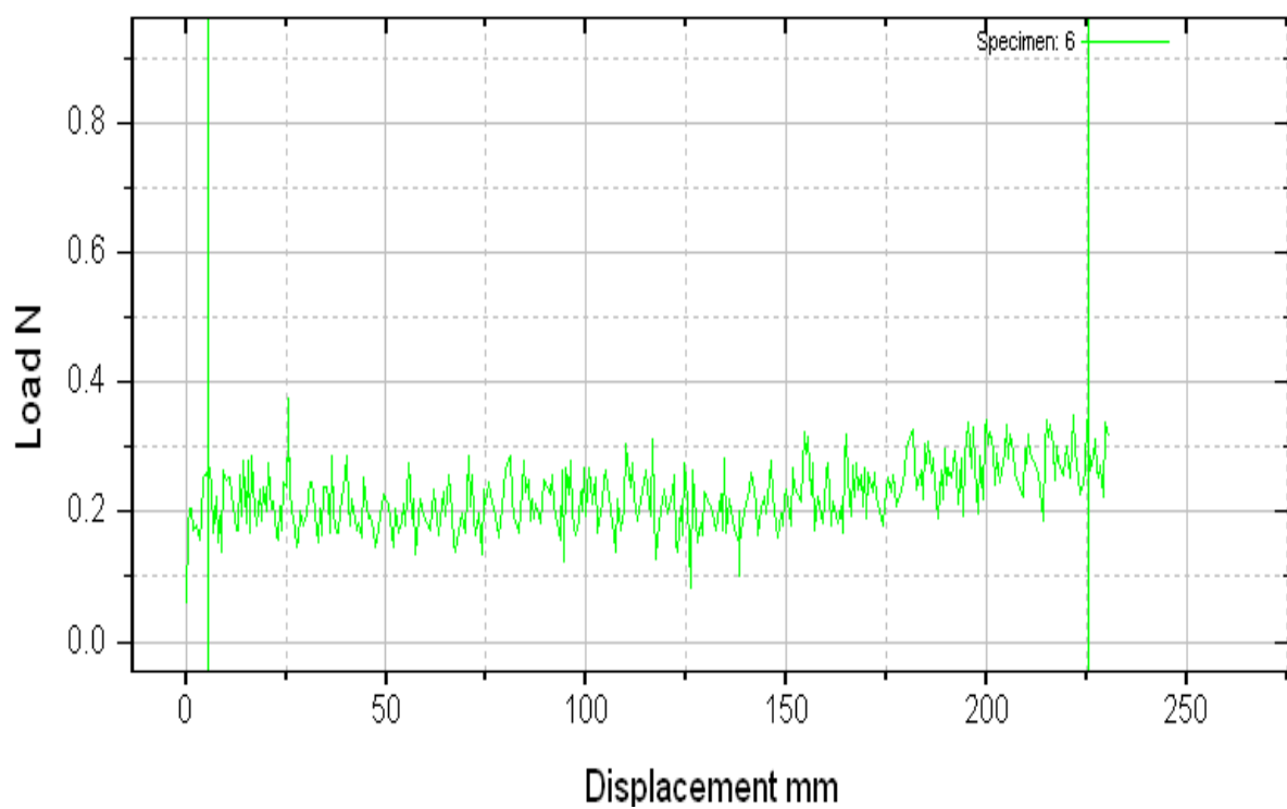
Figure 1(d): A Peel test curve of sample Alk-65 PSA tapes
