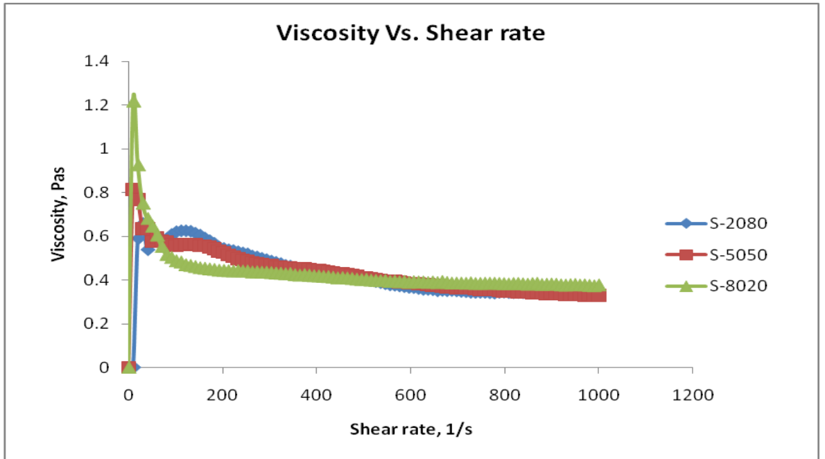
Figure 3: Viscosity Vs. Shear rate for Alk-47 emulsion at different surfactant ratio
