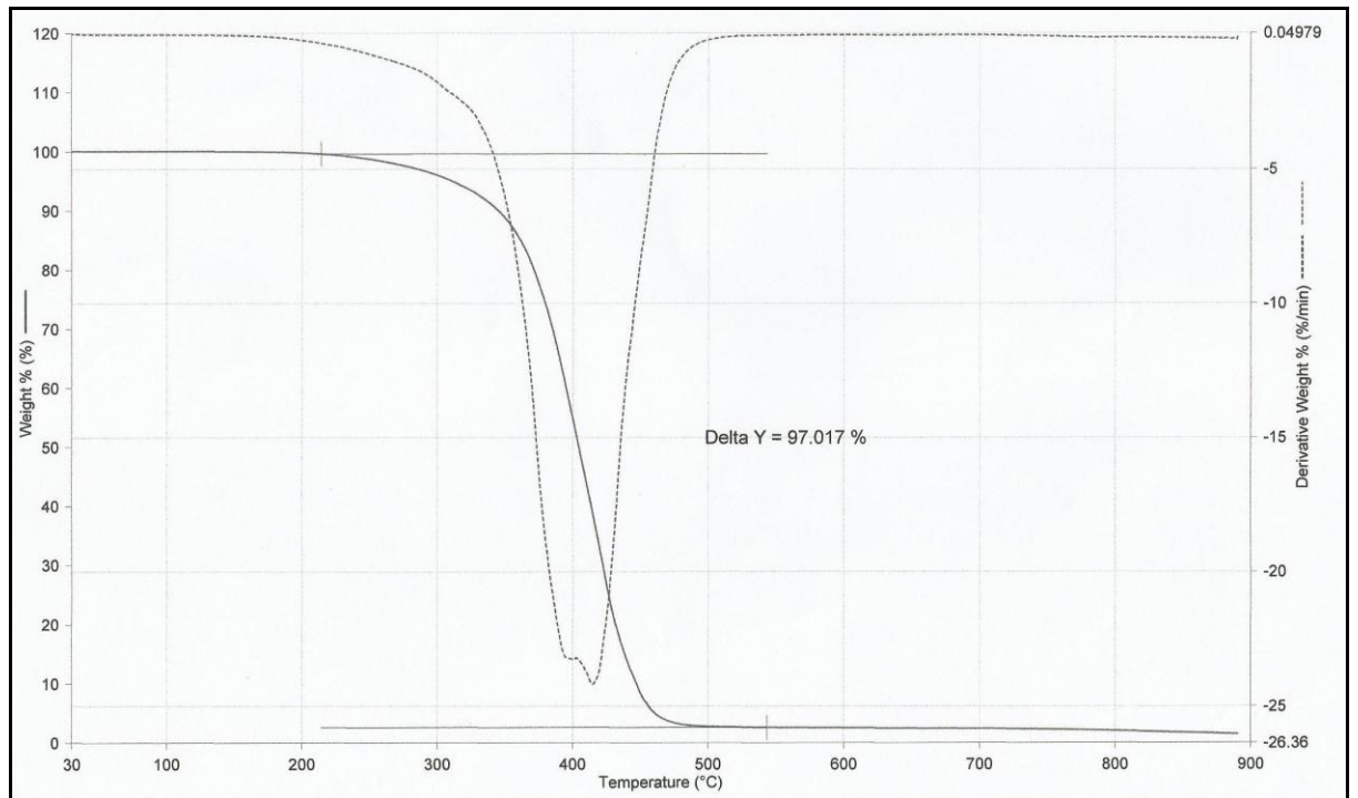
Figure 1: TGA thermogram of Alk-45
