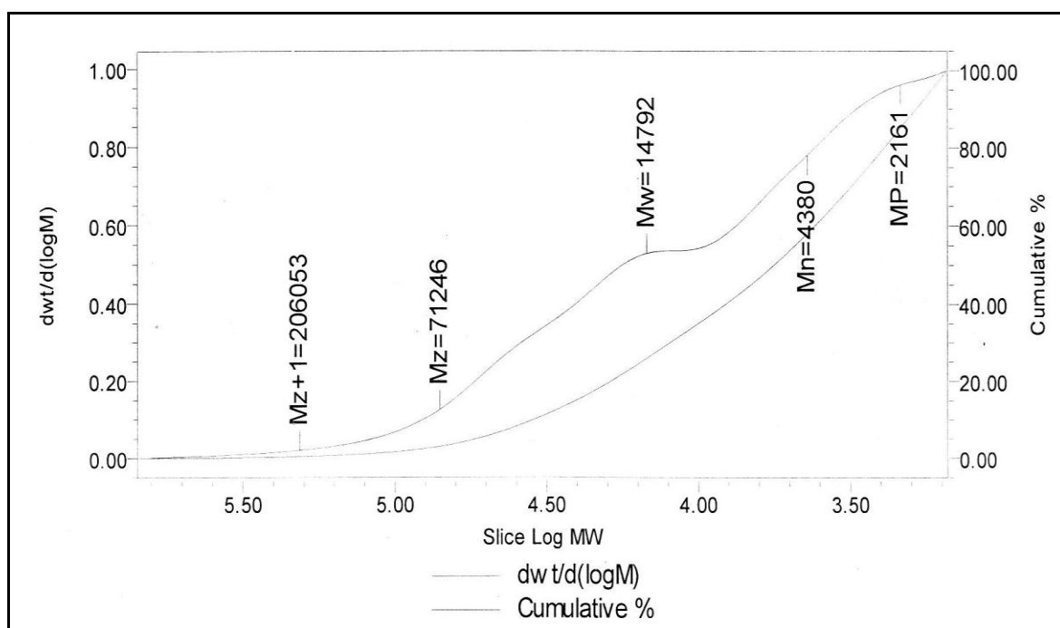
Figure 2: GPC chromatogram of Alk-47
