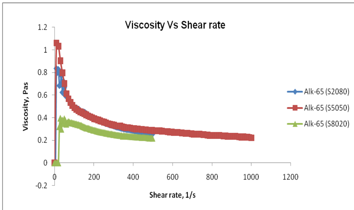
Figure 5: Viscosity Vs Shear rate of Alk-65 emulsion at different surfactant ratio
