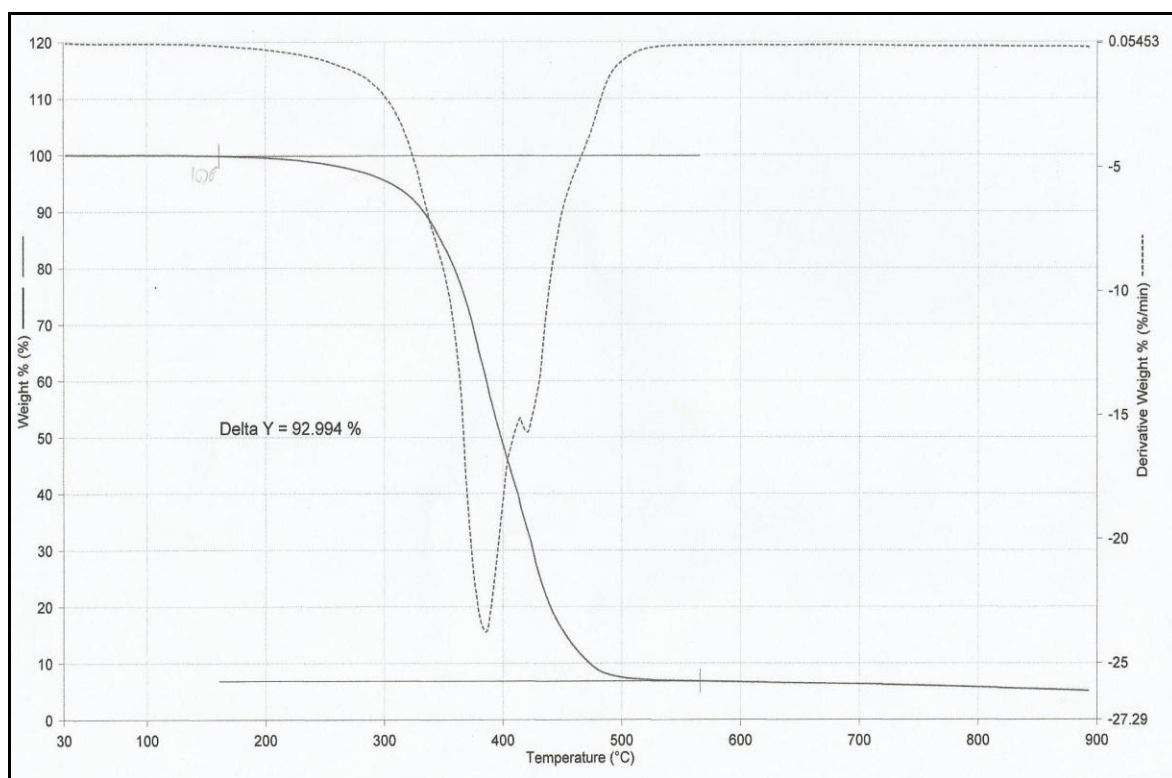
Figure 2: TGA thermogram of Alk-47
