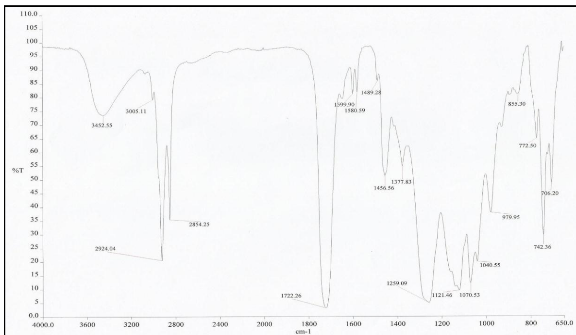
Figure 2: FTIR spectra of Alk-47
