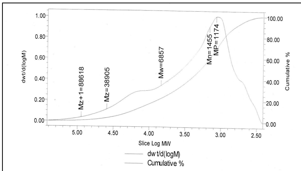
Figure 1: GPC chromatogram of Alk-45
