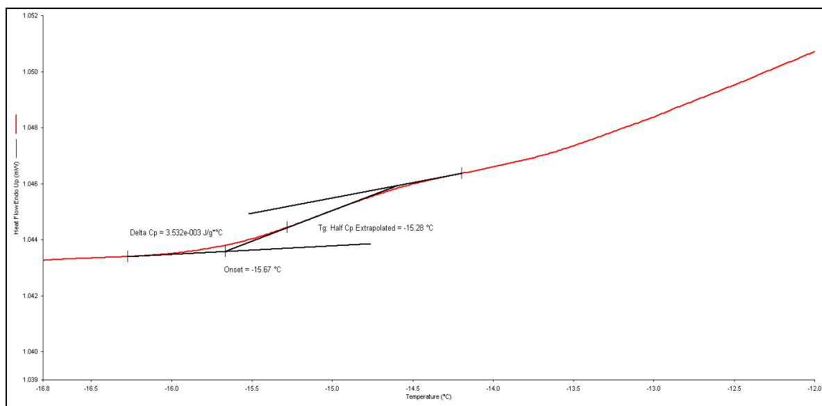
Figure 1: DSC trace of Alk-45
