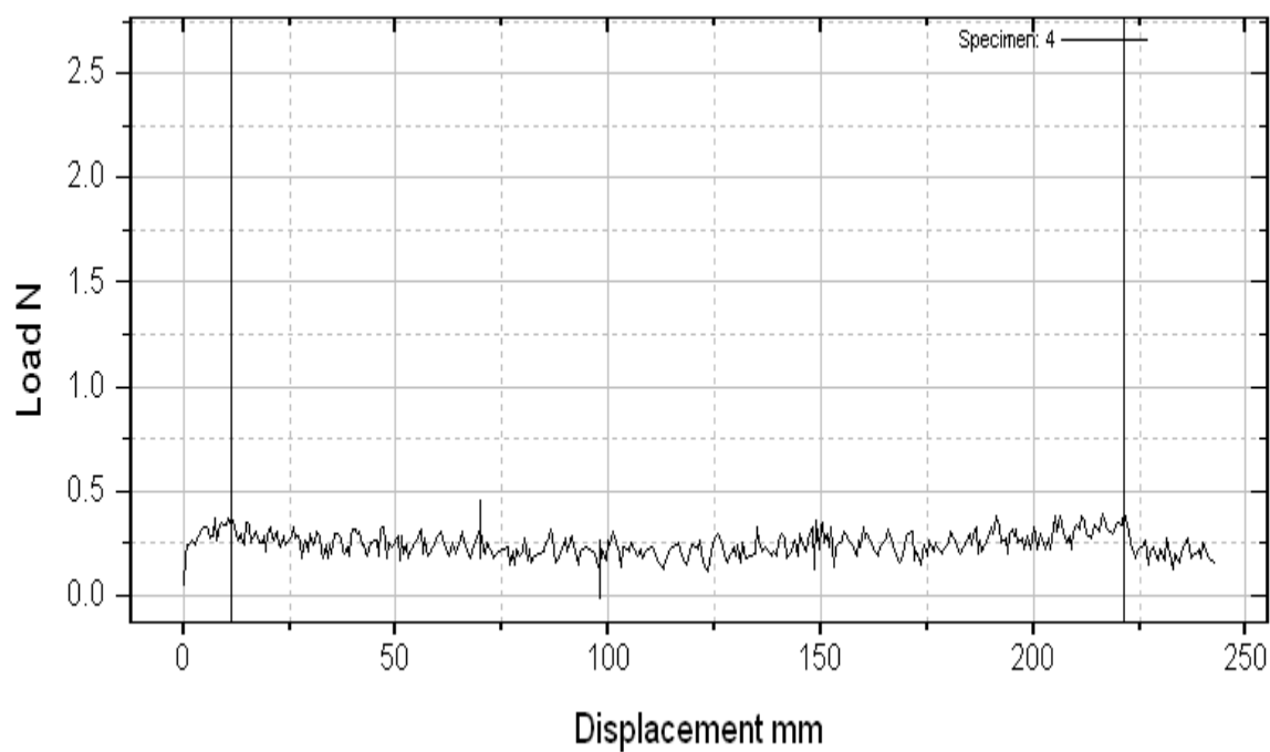
Figure 1(c): A Peel test curve of sample Alk-65 PSA tapes
