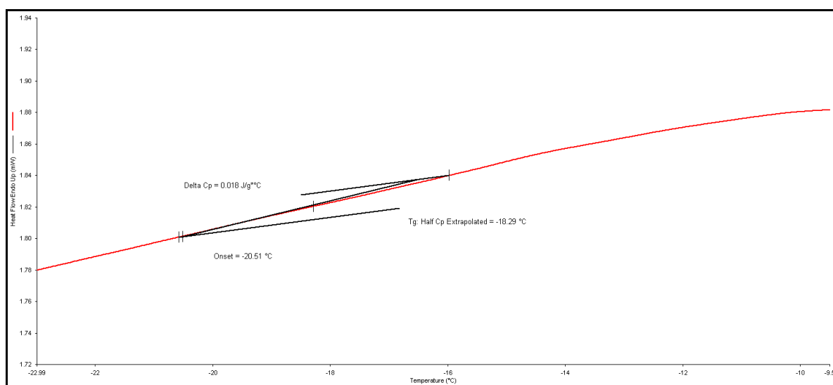
Figure 2: DSC trace of Alk-47
