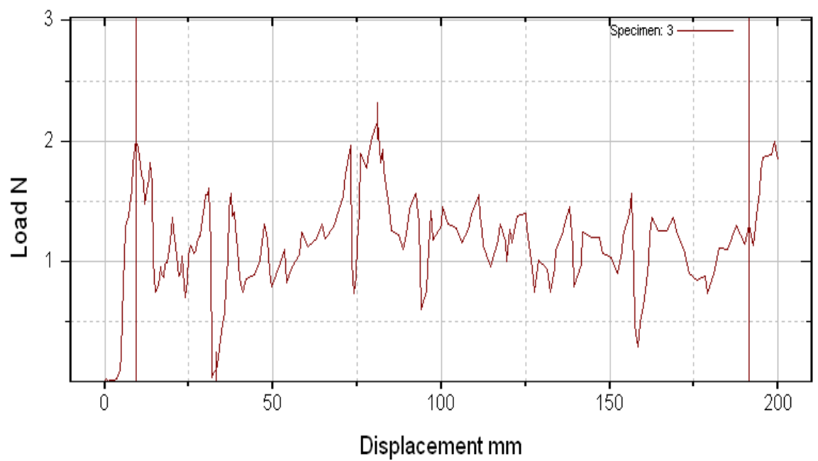
Figure 3(b): A Peel test curve of commercial PSA tapes ESI
