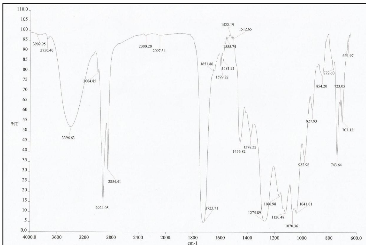
Figure 1: FTIR spectra of Alk-45
