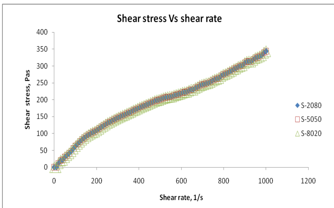
Figure 4: Shear stress Vs. Shear rate for alk-47 emulsion at different surfactant ratio
