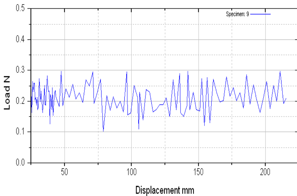
Figure 1(a): A Peel test curve for pure Alk-45
