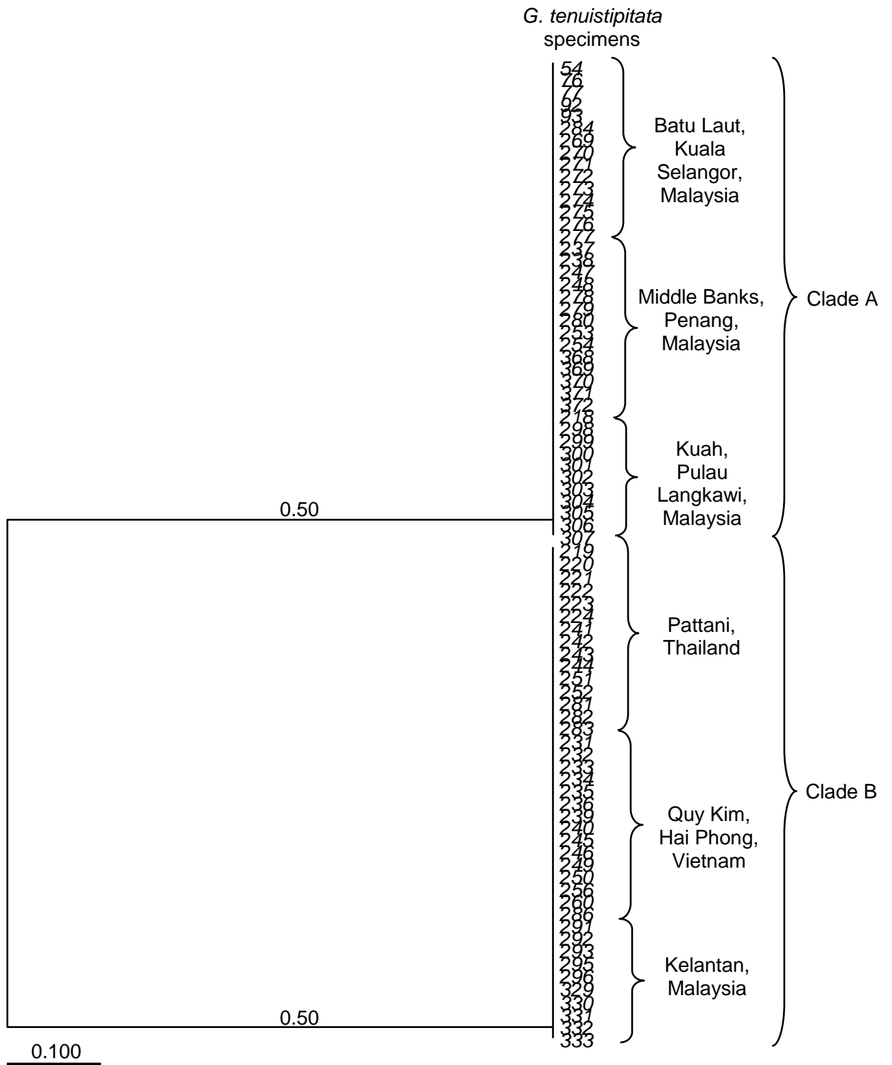
Figure 4.5: Dendrogram generated using the unweighted pair group method with arithmetic average (UPGMA) of eighty G. tenuistipitata specimens from different localities for primer-pair GT8.
