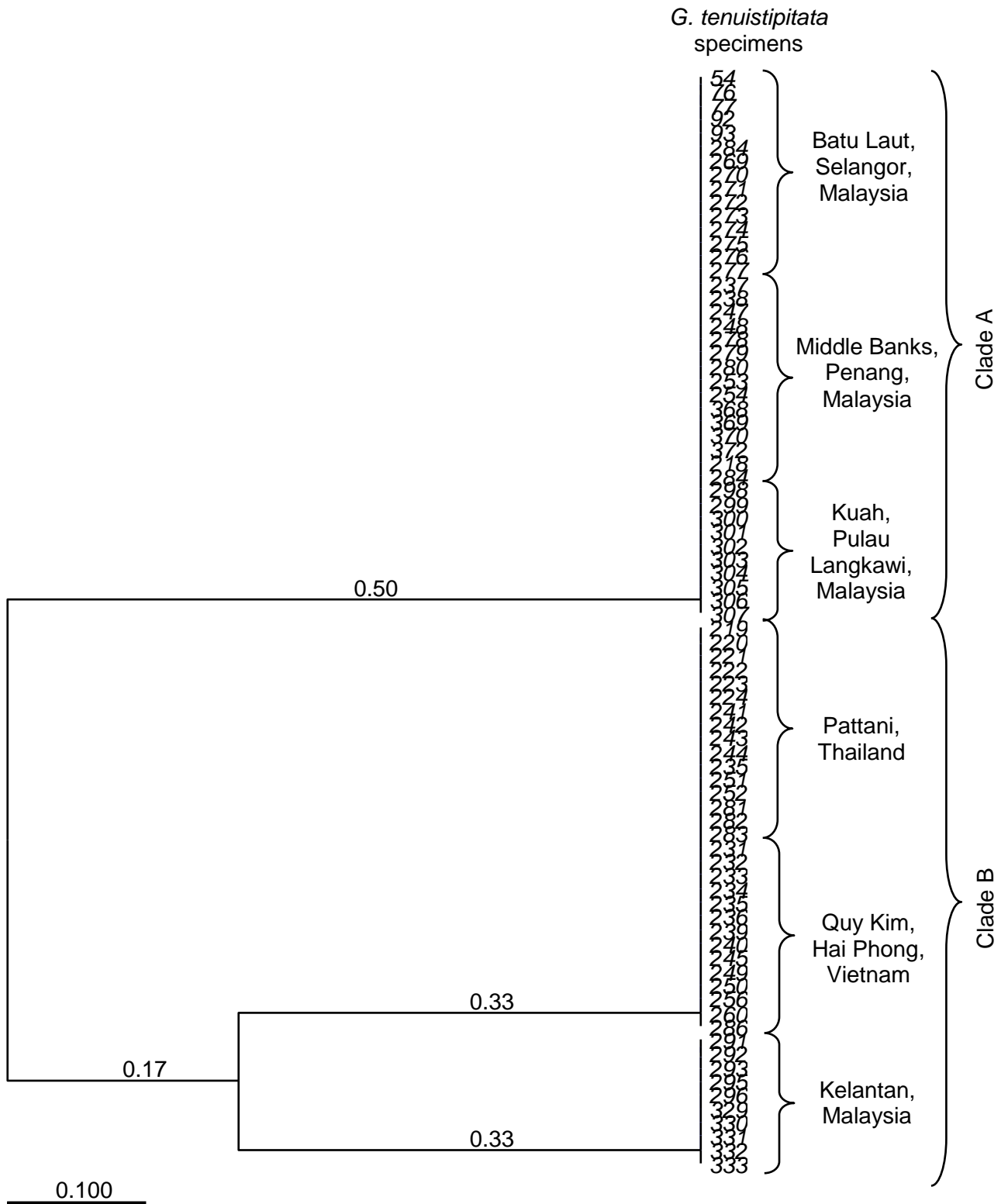
Figure 4.6: Dendrogram generated using the unweighted pair group method with arithmetic average (UPGMA) of eighty G. tenuistipitata specimens from different localities for combined primer-pairs GT5 and GT8.
