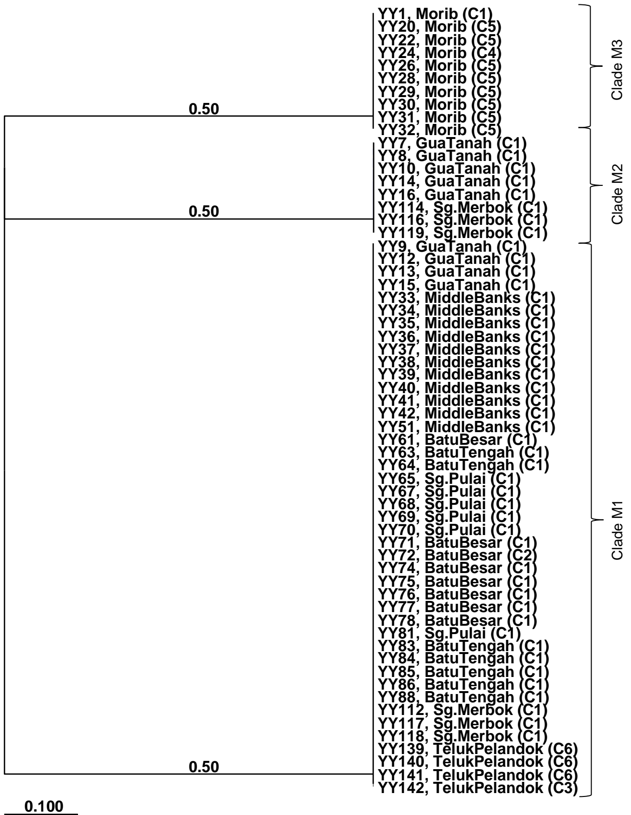
Figure 4.11: Dendrogram generated using the unweighted pair group method with arithmetic average (UPGMA) of Gracilaria changii from Malaysia. The numeric number in bracket after the locality is the haplotype obtained using cox1 gene.
