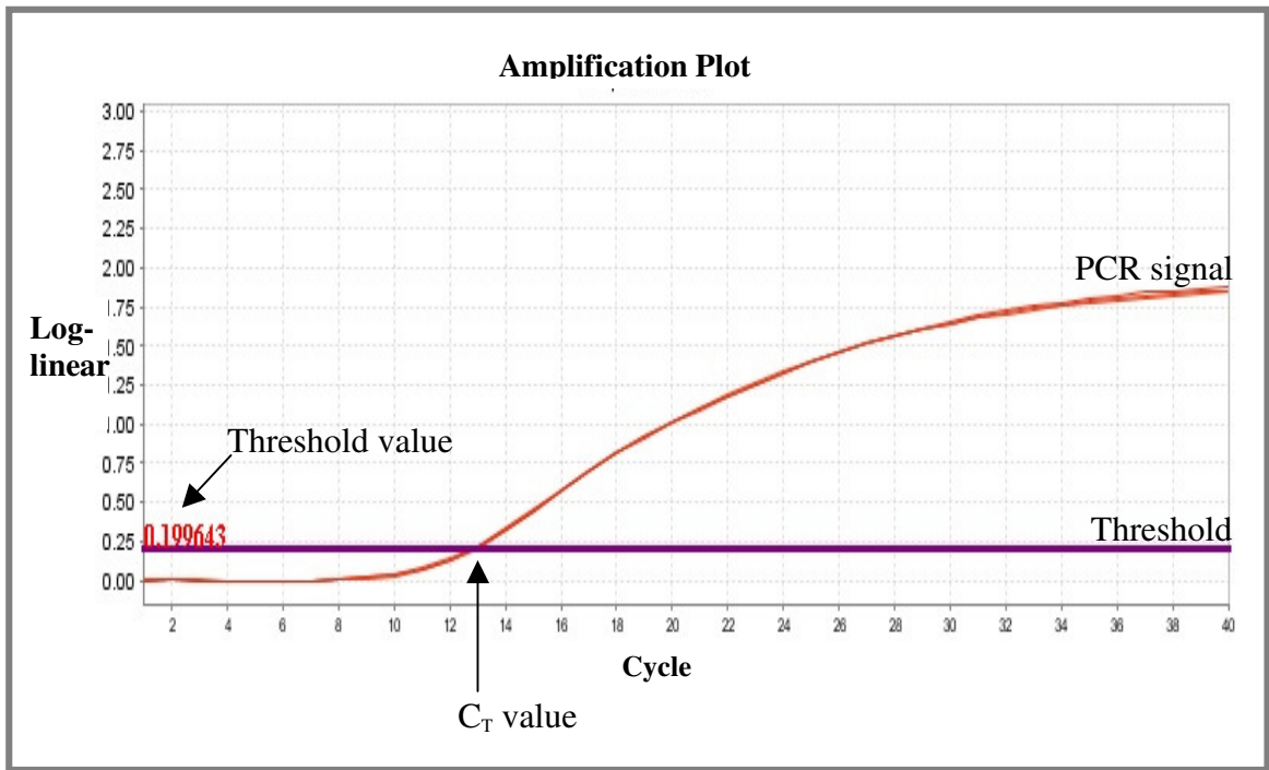
Figure 3.2. Real-time quantitative PCR amplification plot. Amplification plot showing log-linear plot of the PCR signal versus the cycle number. C_T value is determined when the log-linear plot of the PCR signal crosses the threshold value, where replication is at exponential stage.
