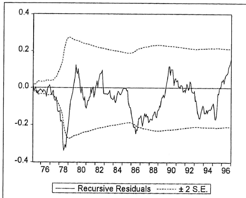
Graph 3.15 Recursive Estimates Stability Test of PPP Model for Japan and United States (based on CPI)
