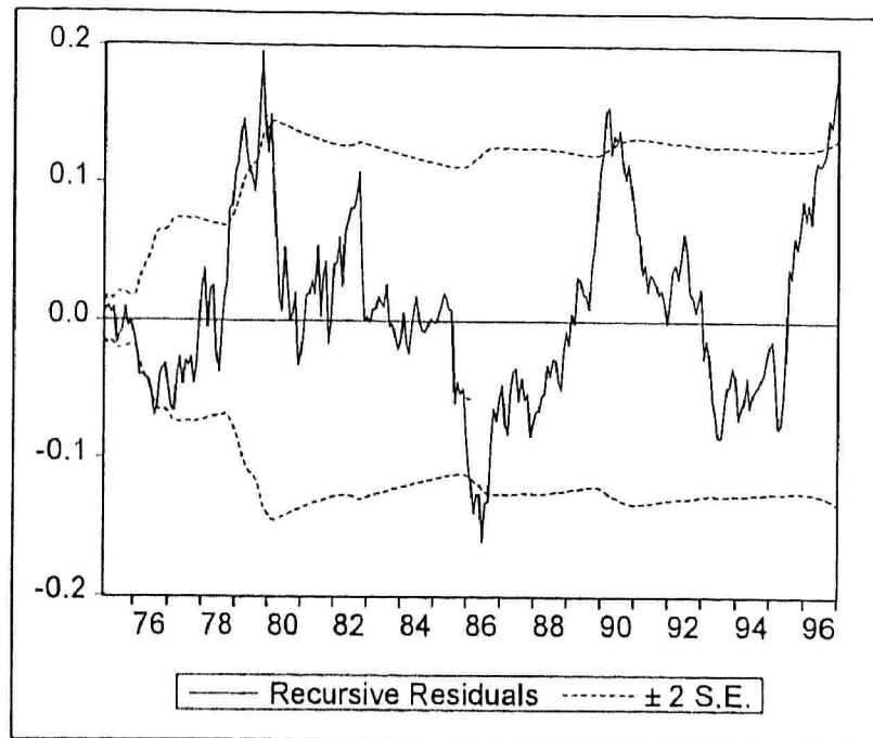
Graph 3.16 Recursive Estimates Stability Test of PPP Model for Japan and United States (based on WPI)
