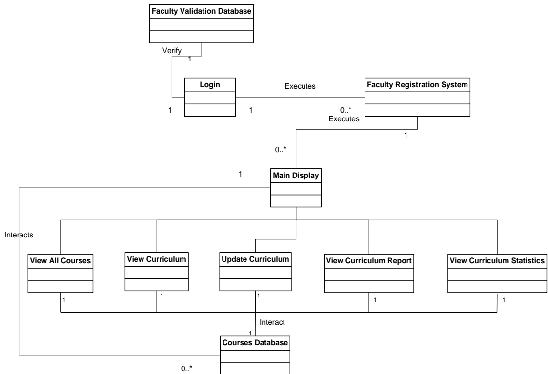
Figure J1: Class diagram for Faculty Registration System
