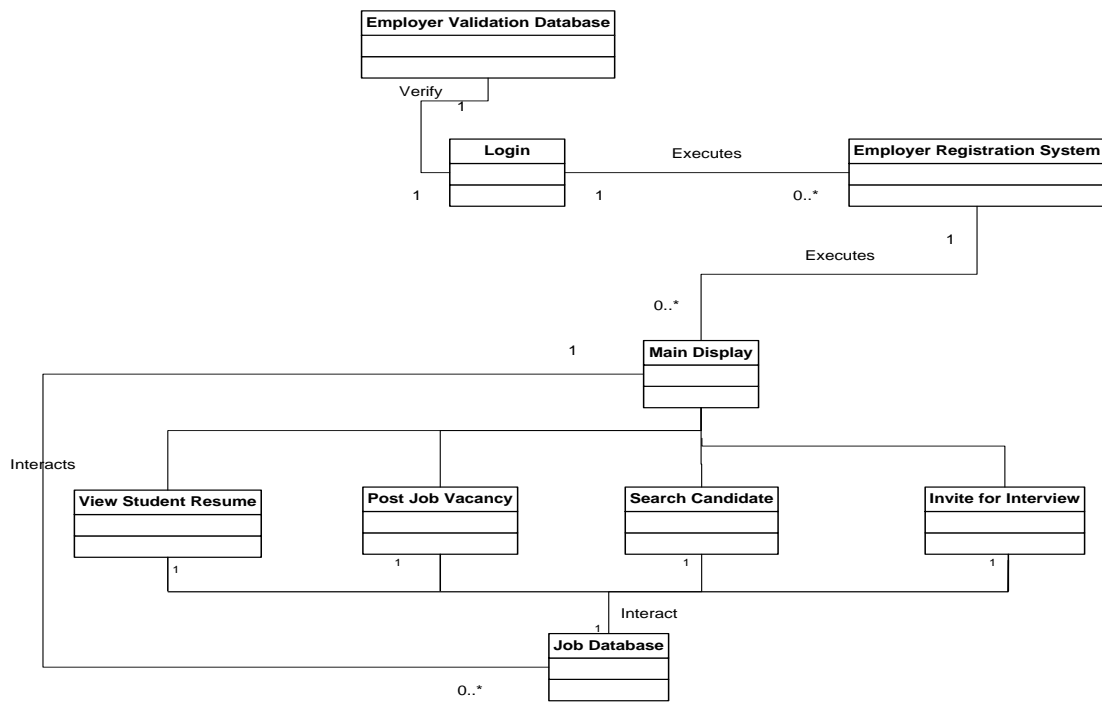
Figure J2: Class diagram for Employer Registration System
