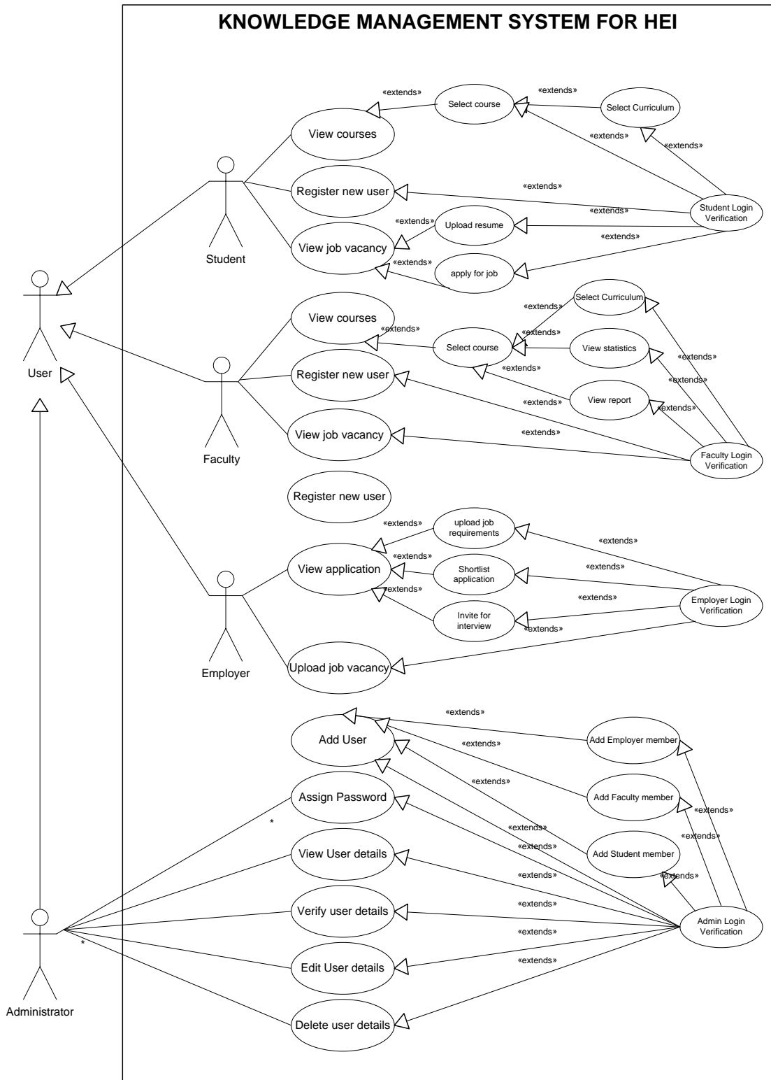
Figure J4: Use Case Diagram for Overall KM in HEI
