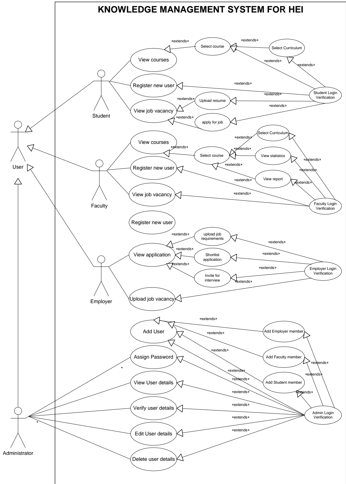
Figure K4; Use Case diagram for the overall KM in HEI.
