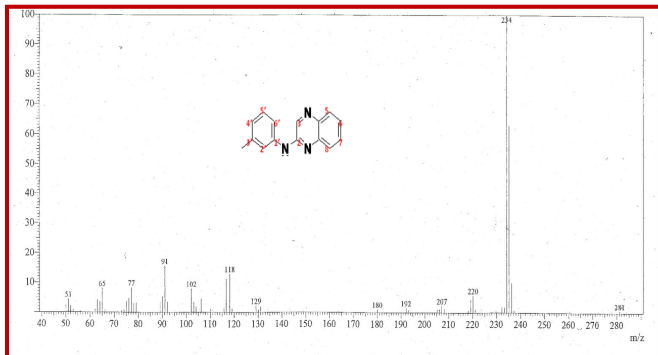
GCMS spectrum of 2-N-(m-Methyl)anilinoquinoxaline (L6)
