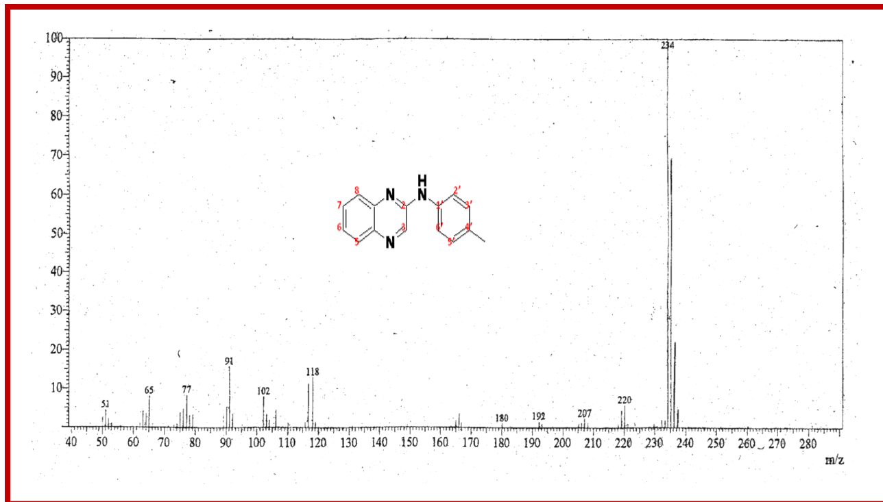
GCMS spectrum of 2-N-(p-Methyl)anilinoquinoxaline (L7)
