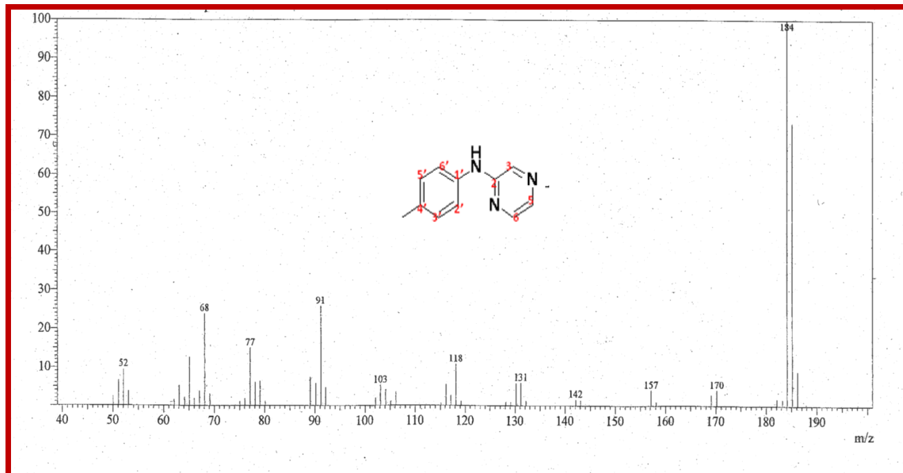
GCMS spectrum of 2-N-( p -Methyl)anilinopyrazine (L3)
