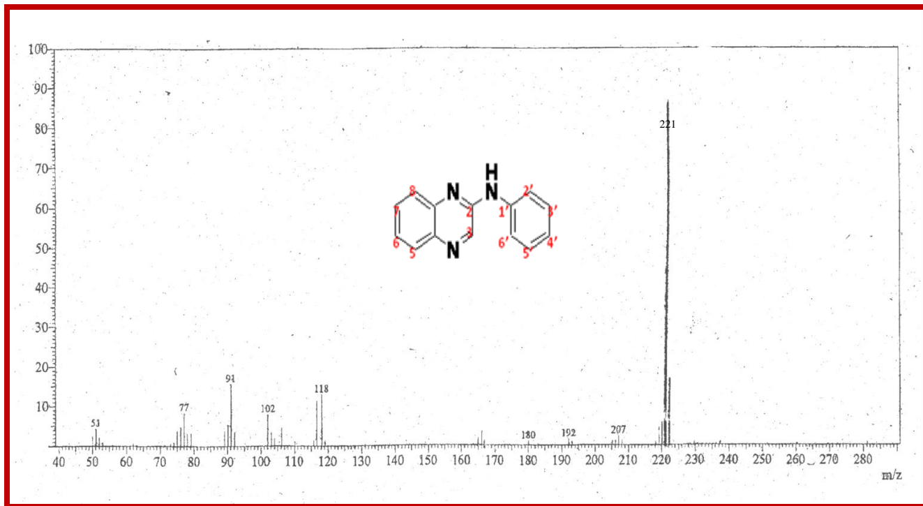
GCMS spectrum of 2-N-Anilinoquinoxaline (L5)
