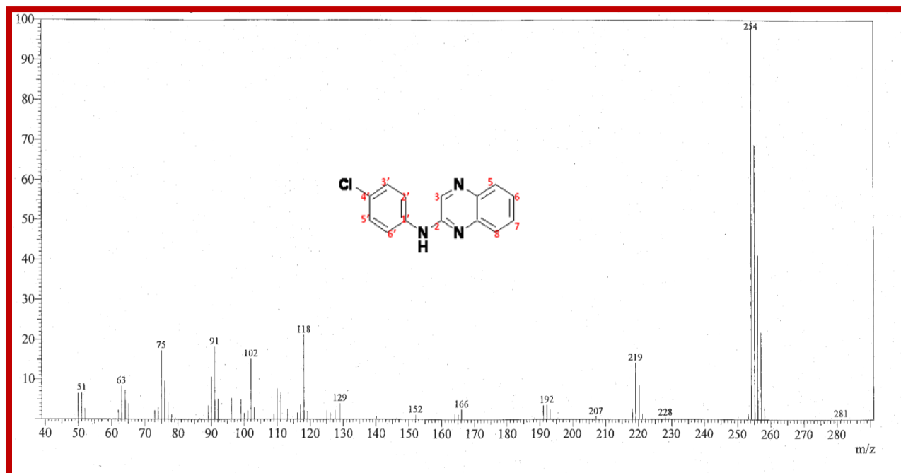
GCMS spectrum of 2-N-(p-Chloro)anilinoquinoxaline (L8)
