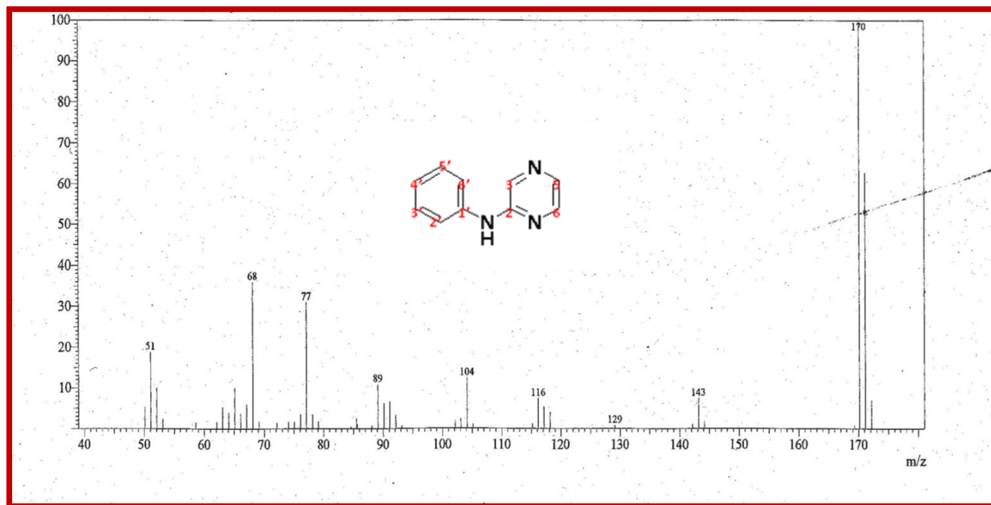
GCMS spectrum of 2-N-Anilinopyrazine (L1)
