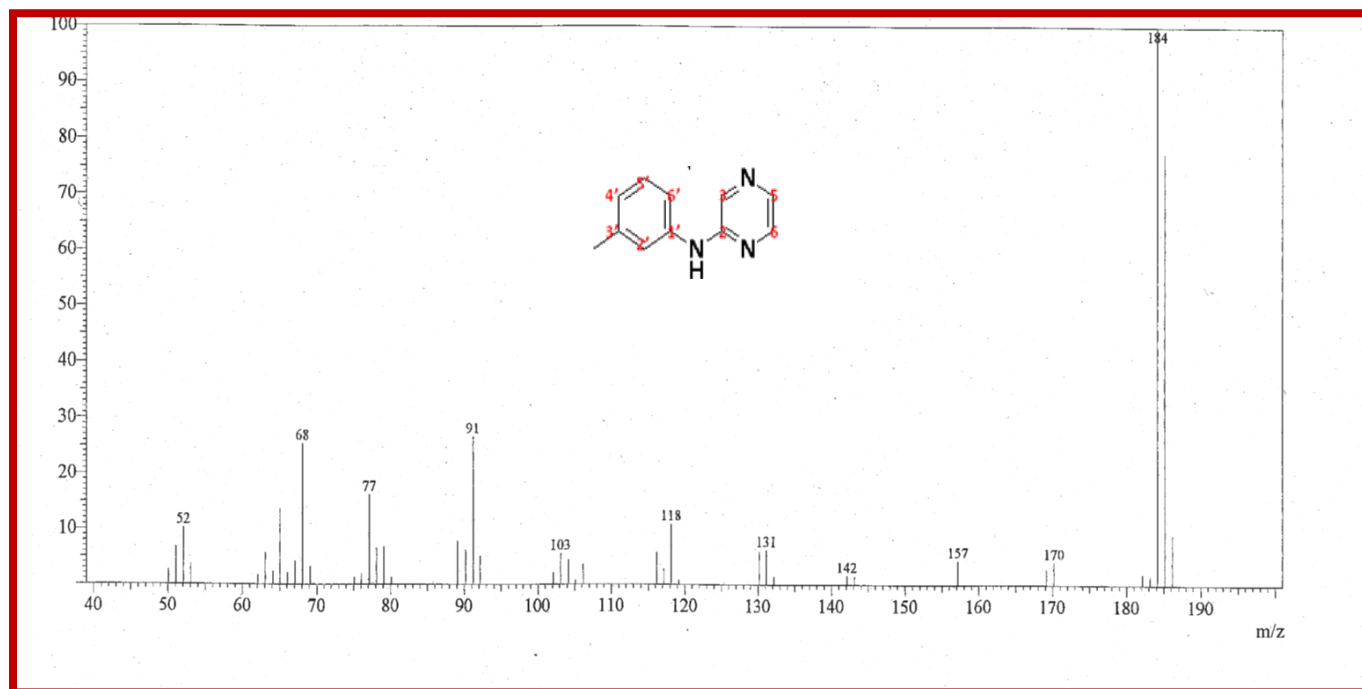
GCMS spectrum of 2-N-(m-Methyl)anilinopyrazine (L2)
