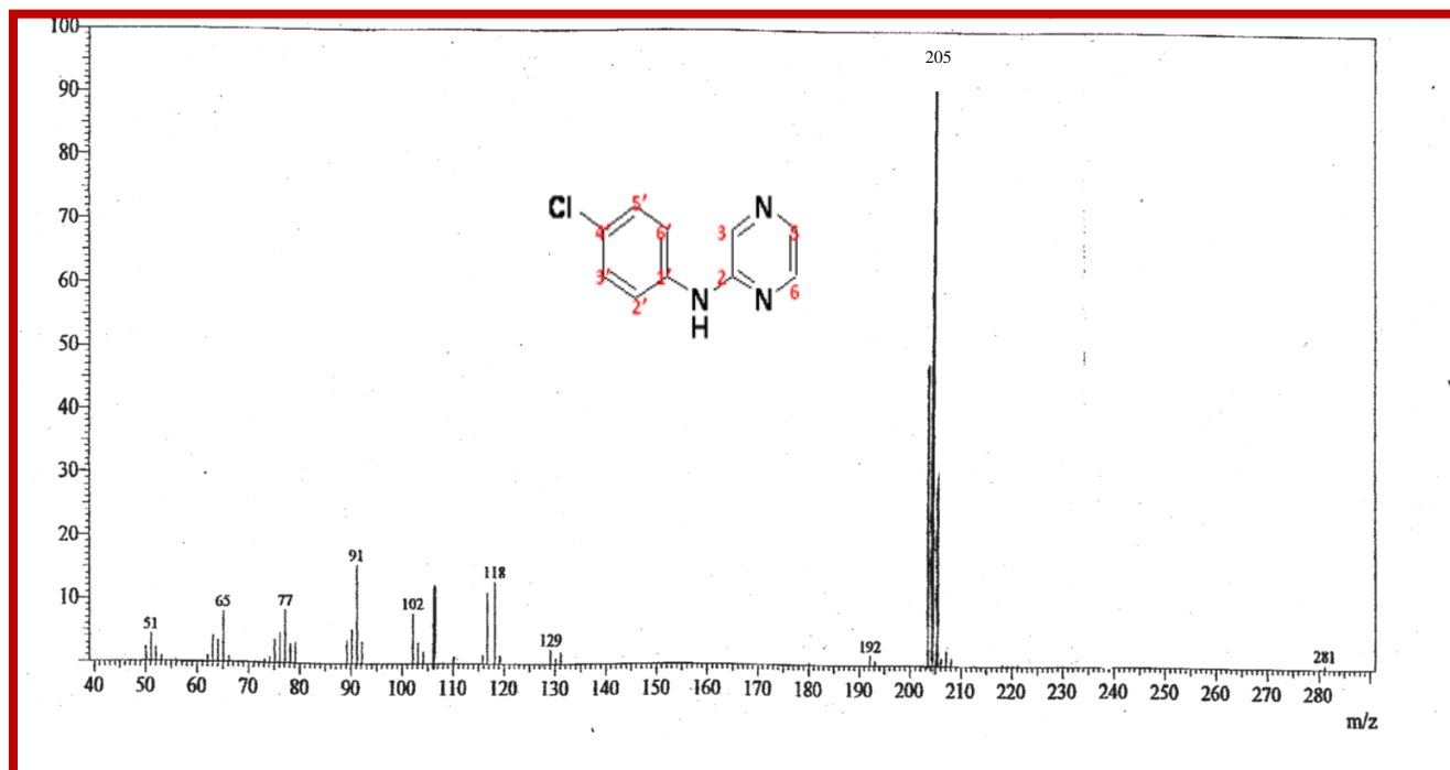
GCMS spectrum of 2-N-( p -Chloro)anilinopyrazine (L4)
