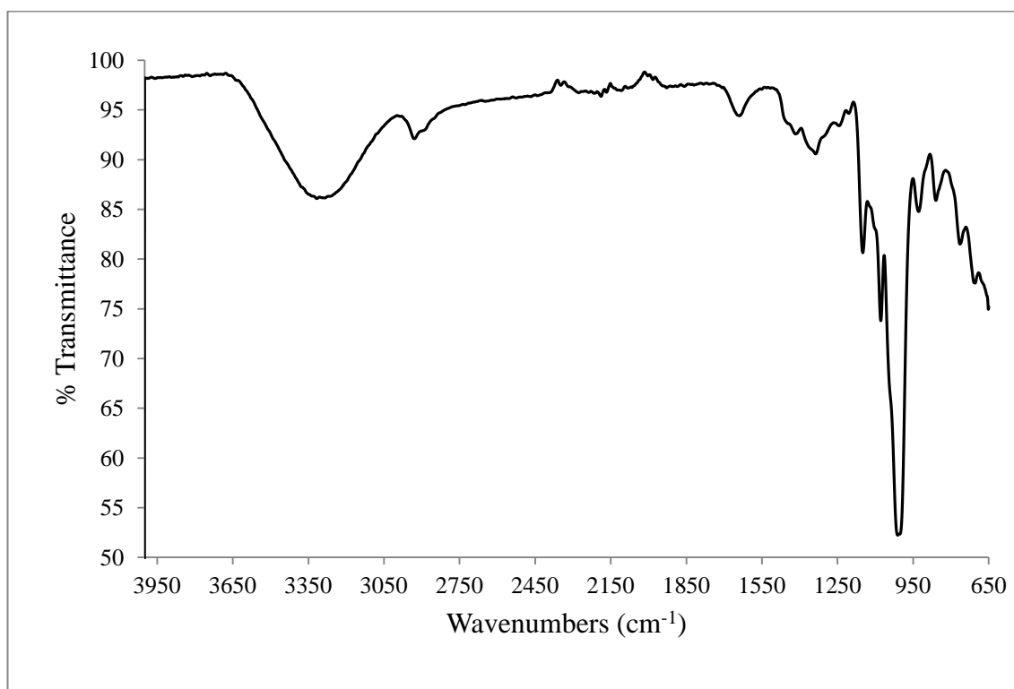
FTIR spectrum of pure rice starch in the frequency range of 650-4000 \text{cm}^{-1}
