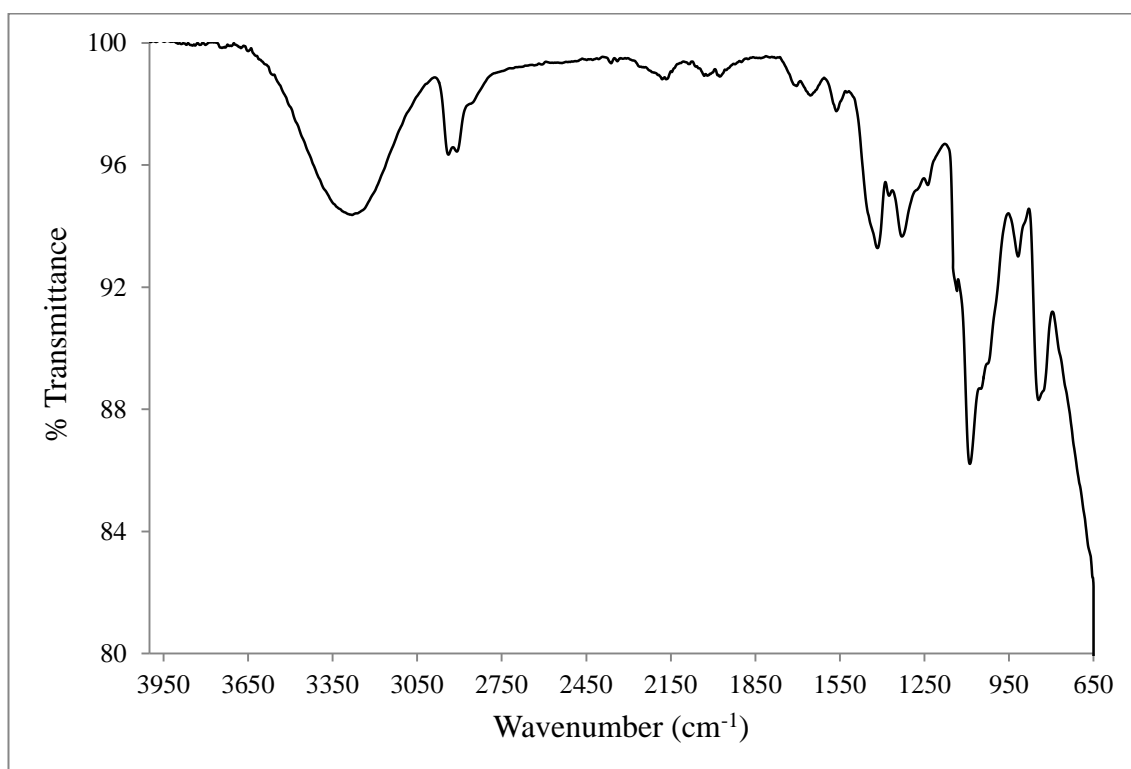
FTIR spectrum of PVA/ITS in the frequency range of 650-4000 \text{cm}^{-1}
