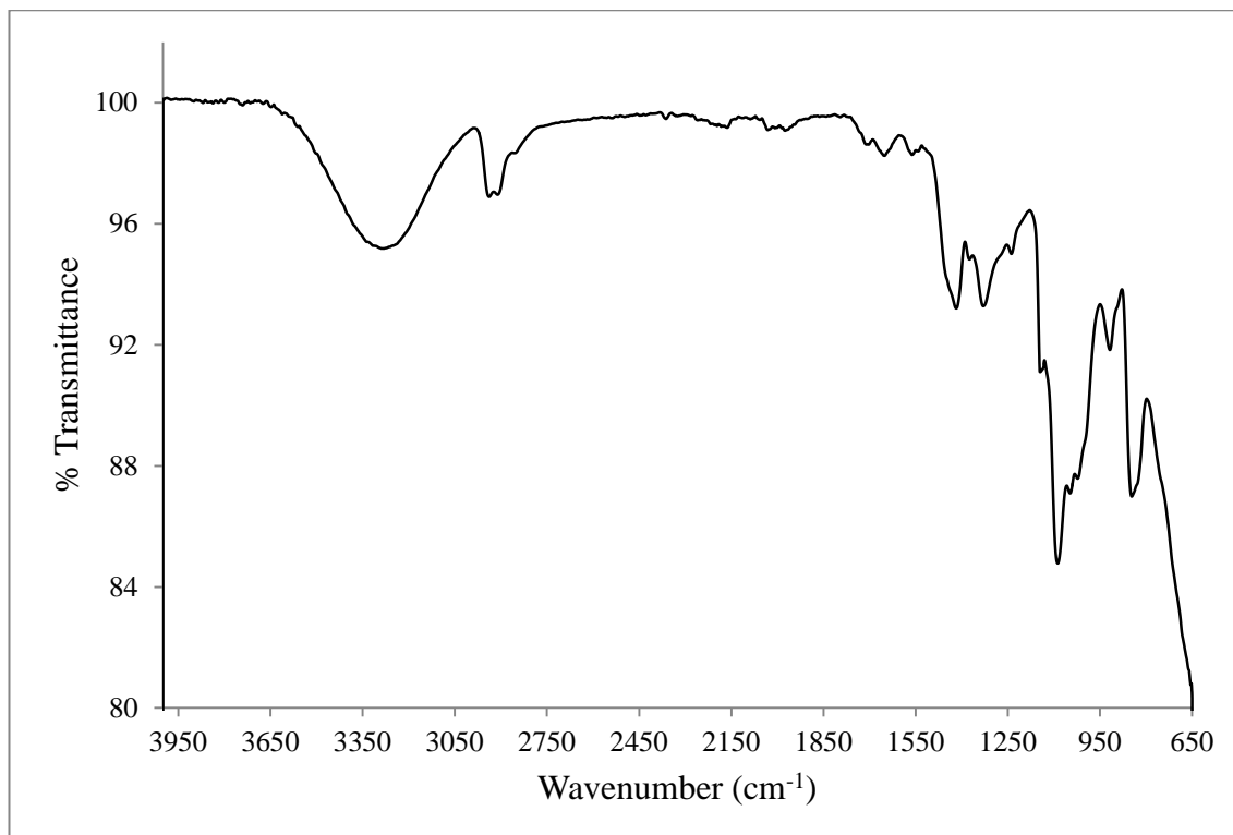
FTIR spectrum of PVA/3TS in the frequency range of 650-4000 \text{cm}^{-1}
