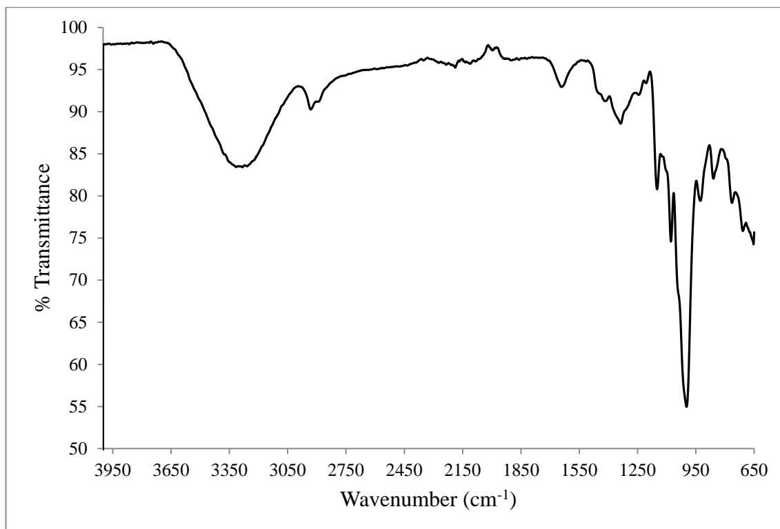
FTIR spectrum of pure tapioca starch in the frequency range of 650-4000 \text{cm}^{-1}
