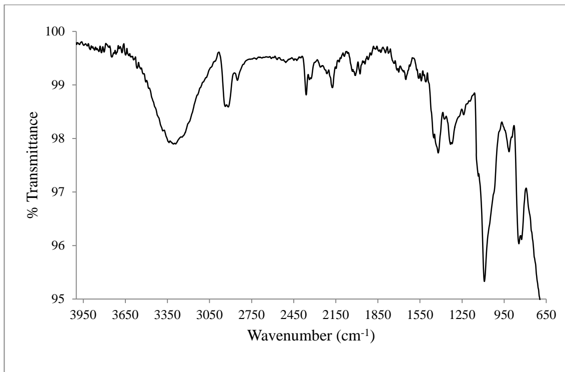
FTIR spectrum of PVA/3SS in the frequency range of 650-4000 cm -1
