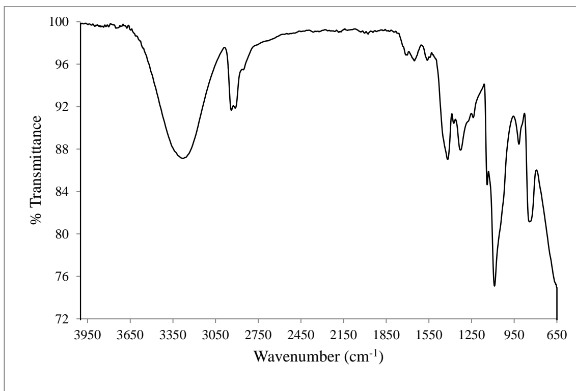
FTIR spectrum of PVA/3RS in the frequency range of 650-4000 cm -1
