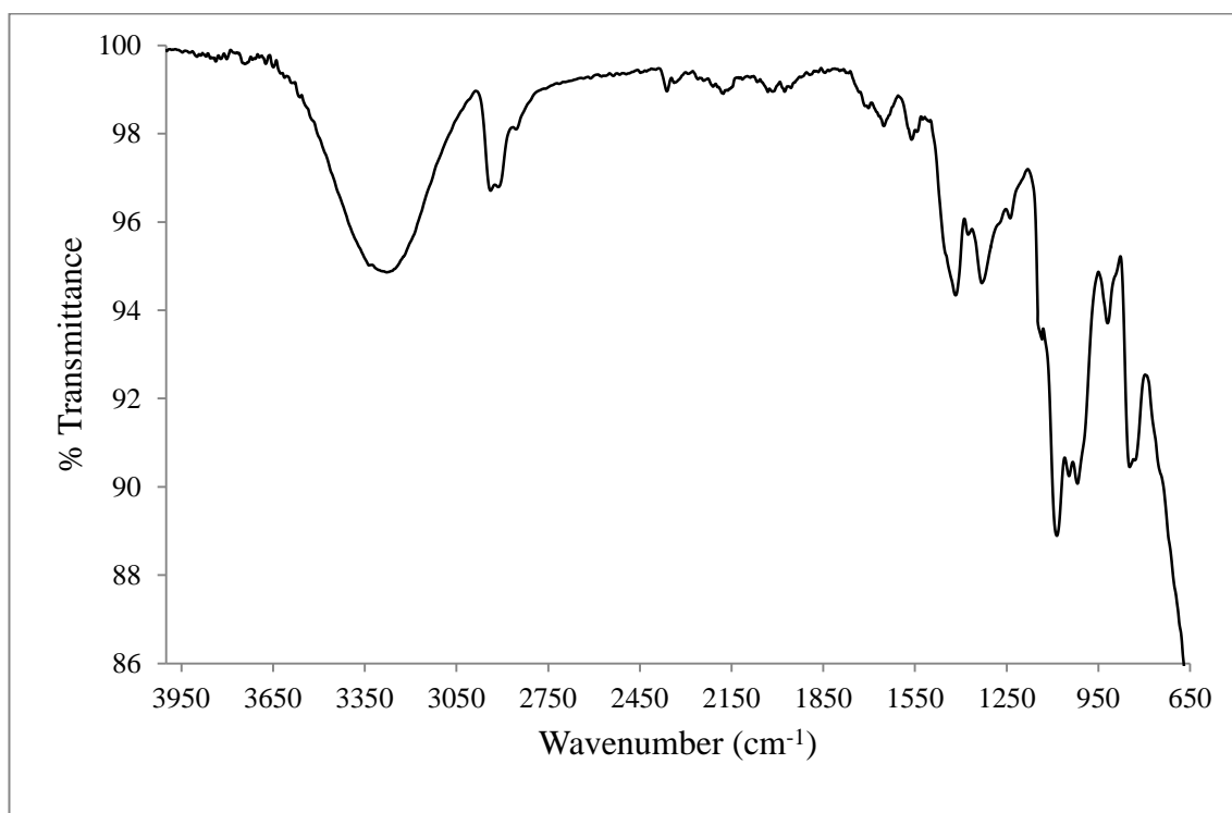
FTIR spectrum of PVA/ISS in the frequency range of 650-4000 \text{cm}^{-1}
