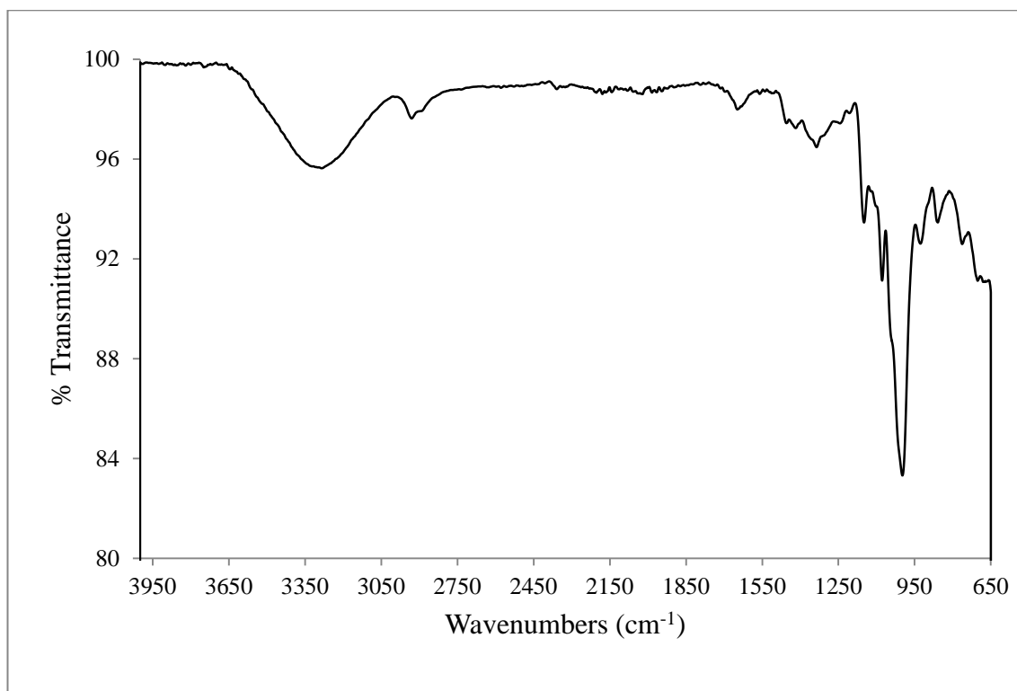
FTIR spectrum of pure sago starch in the frequency range of 650-4000 \text{cm}^{-1}
