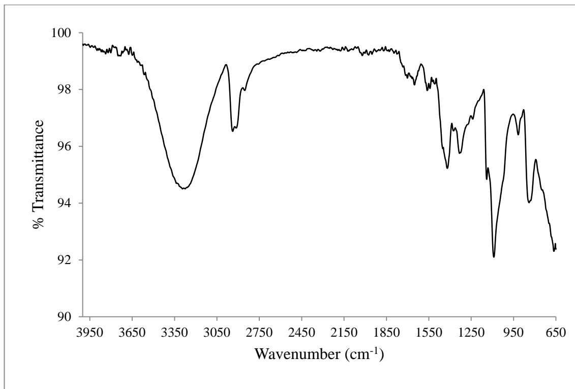
FTIR spectrum of PVA/1RS in the frequency range of 650-4000 cm -1
