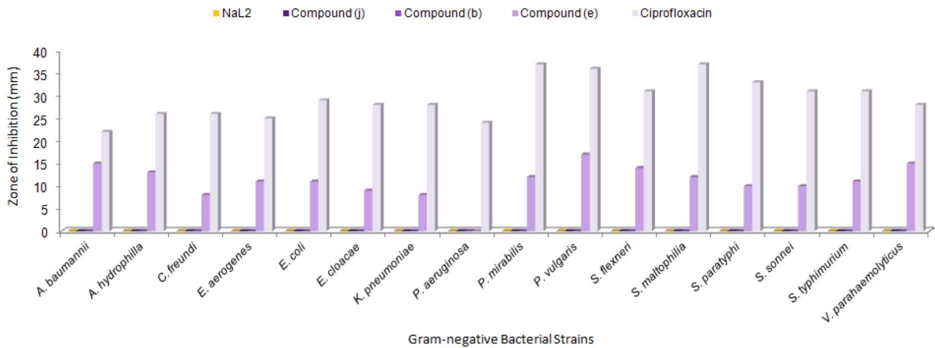
Figure 3.1: Inhibitory activity against Gram-negative bacterial strains measured by zone of inhibition (mm) by NaL2 and its gold(I) complexes; (j), (b) and (e) with ciprofloxacin as the standard drug.
