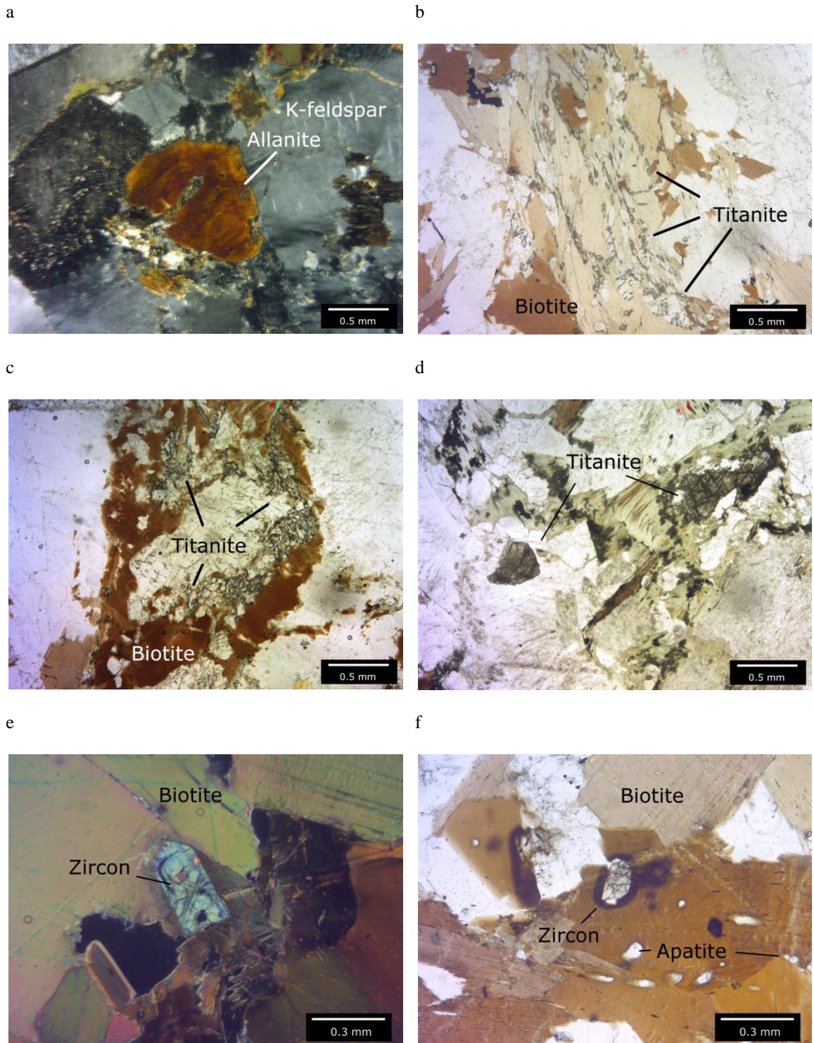
Fig. 4.5: Thin section photomicrograph of melagranite (a) allanite in cross nicols light, (b) tiny titanite grain within a group of biotite, (c) tiny titanite grain within a group of biotite, (d) near euhedral, fragmented titanite in a heavily chloritized biotite, (e) large zircon grain, (f) zircon and apatite accessory within biotite group. Scale bar is shown on the bottom right of the picture.
