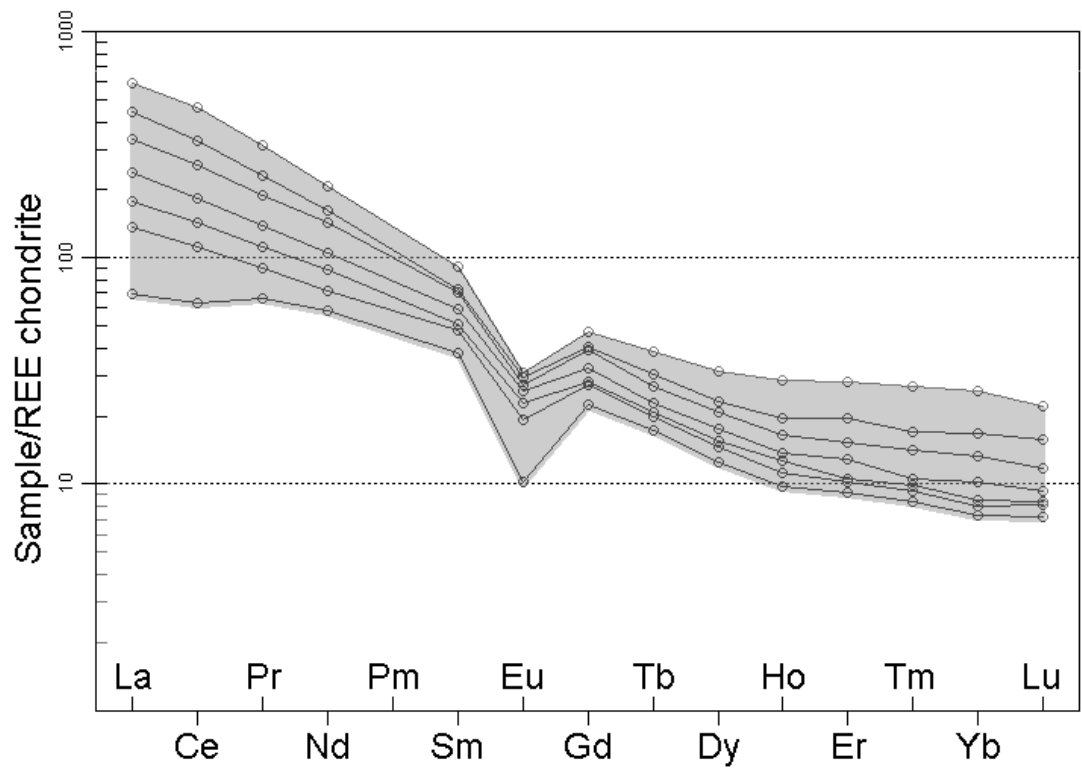
Fig. 5.3: Melagranite Boynton (1984) Chondrite normalized REE plot
