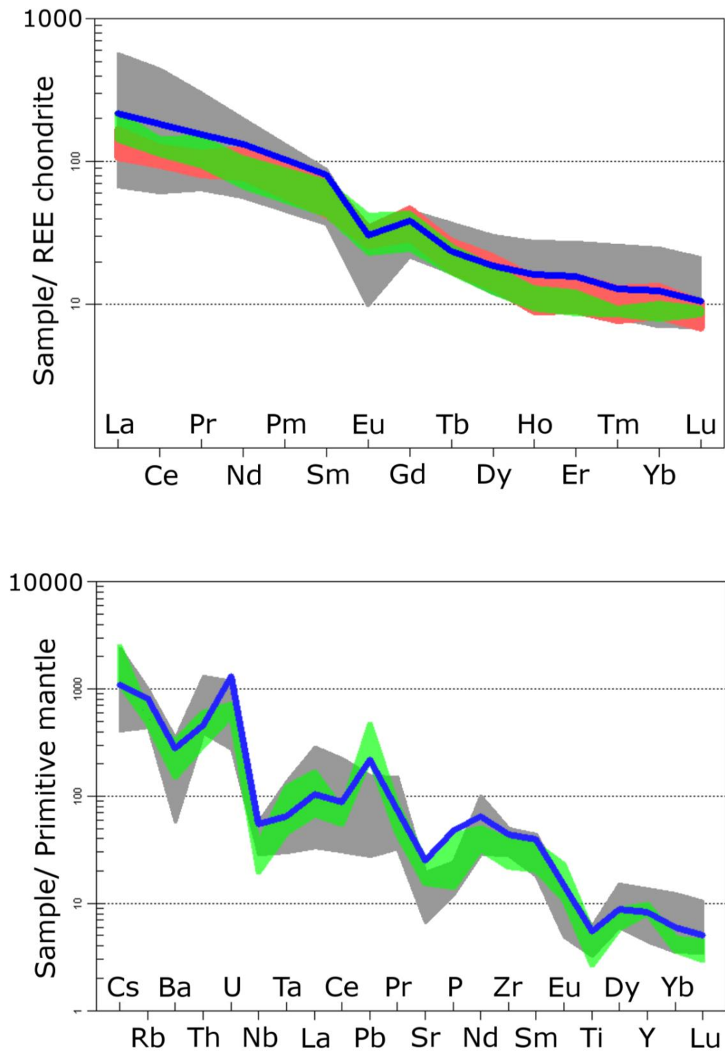
Fig. 5.7: Durbachite series comparison. Top: Boynton (1984) Chondrite normalized REE plot. Bottom: McDonough and Sun (1995) Primitive mantle normalized multi element diagram. Grey: Taiping “durbachite”; Blue: Trebic mafic durbachite (1 sample, melagranite) from Kotkova et al. (2010); Green: Certovo Bremeno suite from Janousek et al. (2000); Red: Bowes and Kosler (1993) durbachite.
