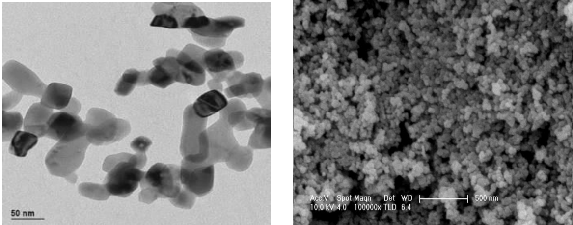
Fig.4.1 SEM micrographs of TiO 2 nanoparticles which originally in dispersed form supplied by Siquist Technology
