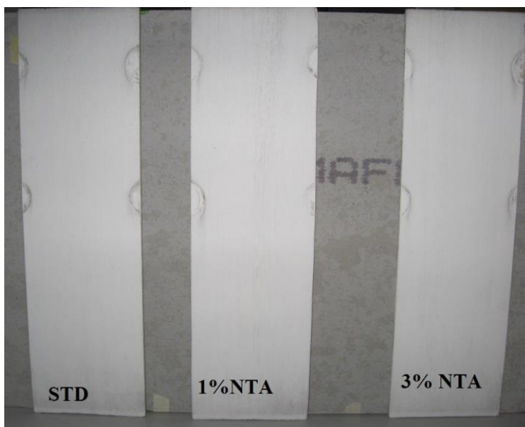
Fig.4.4 Dirt streak marks on panels painted with STD, 1%NTA and 3%NTA after 4 months exposure on 90° rack with slits.
