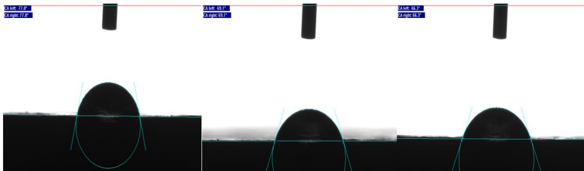
Fig. 4.2 Water contact angle measurements for coatings on a fiber cement substrate: (a) STD; (b) 1% NTA ;(c) 3% NTA
