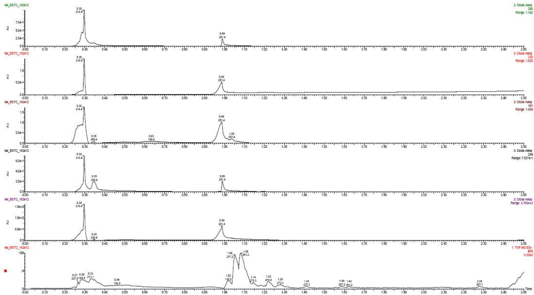
Figure 4.31 : LC-MS chromatogram of N 4 sample.
