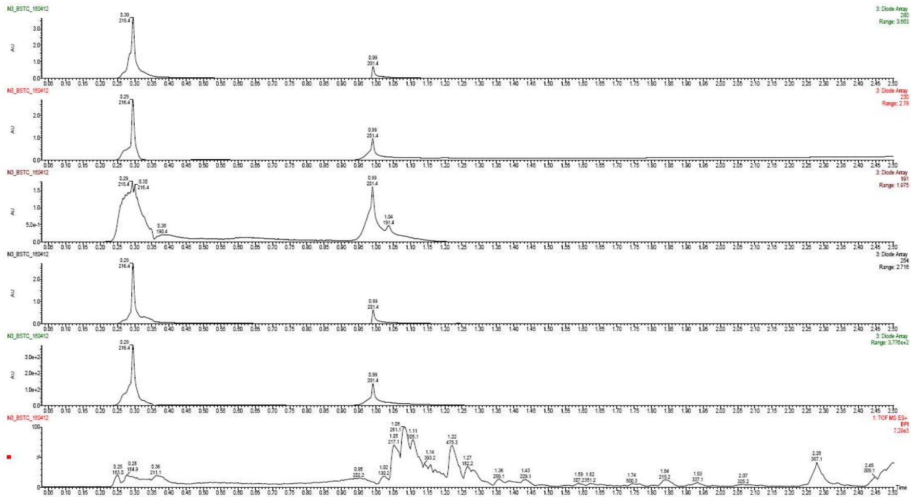
Figure 4.29 : LC-MS chromatogram of N 3 sample.
