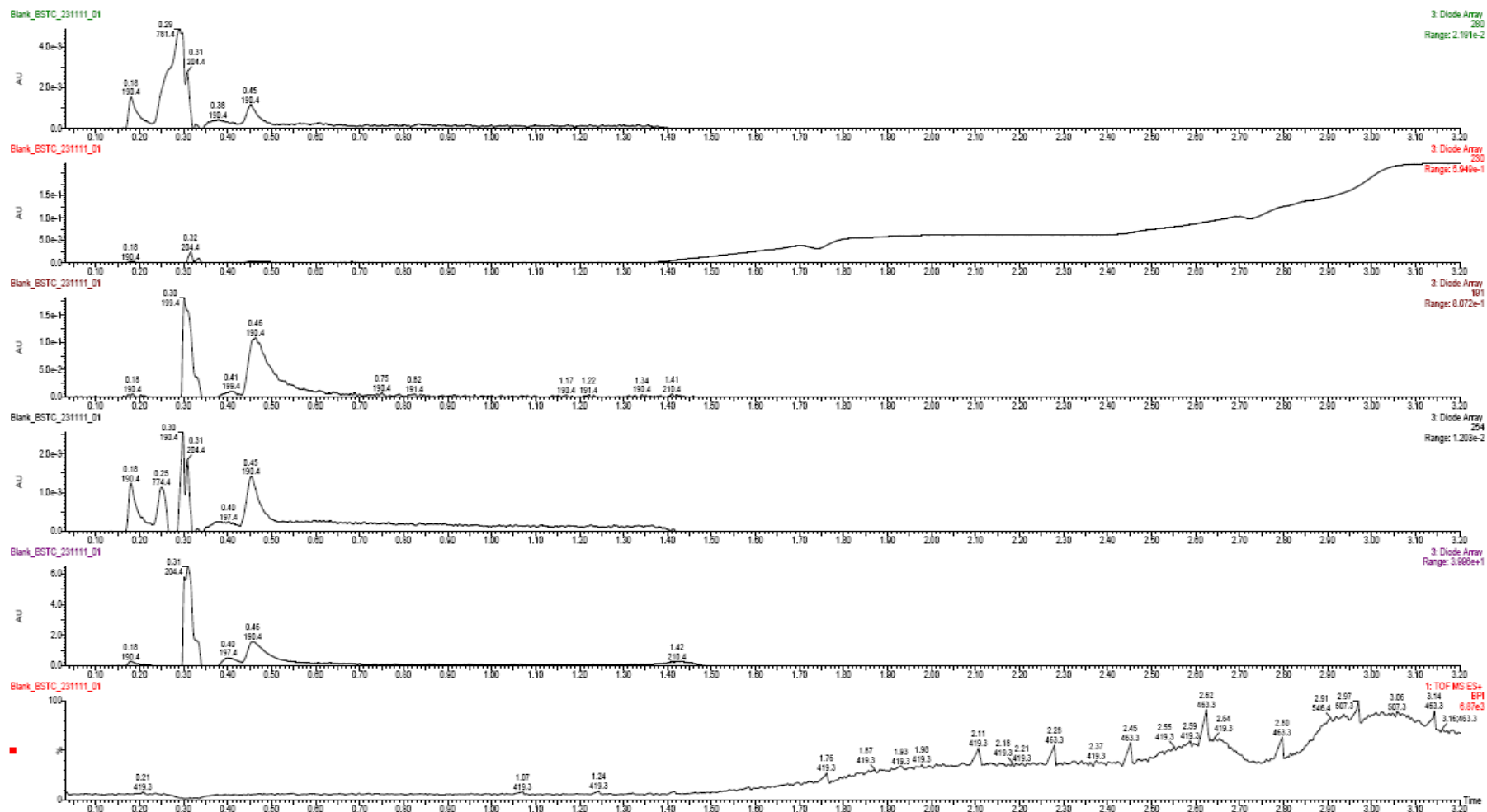
Figure 4.28 : Blank for LC-MS.
